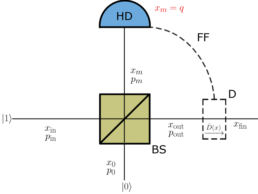
Figure III.2: Schematic depiction of CV quantum erasing. HD is the homodyne detector. FF is the feed-forward and D is displacement where the displacement operation ( \hat{D}(x) ) takes place. The measured position quadrature is marked q
