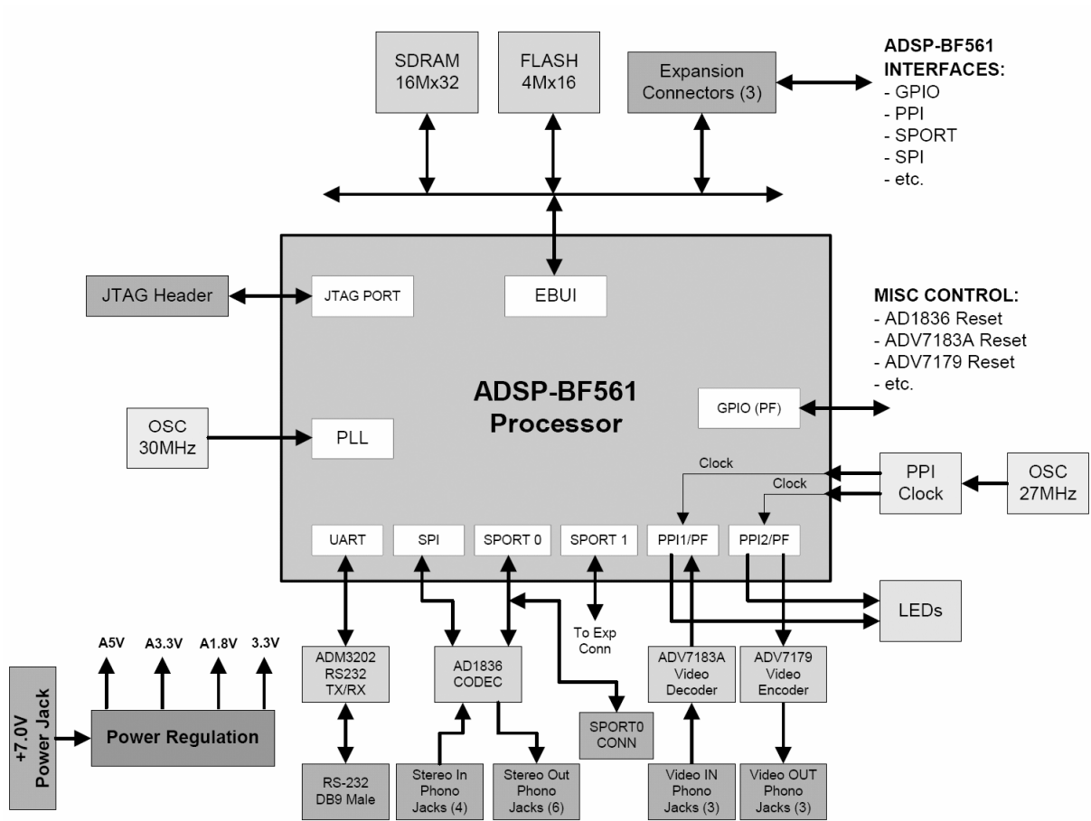
Figure 8: Development board EZ-KIT Lite® ADSP-BF561 - System Architecture.
