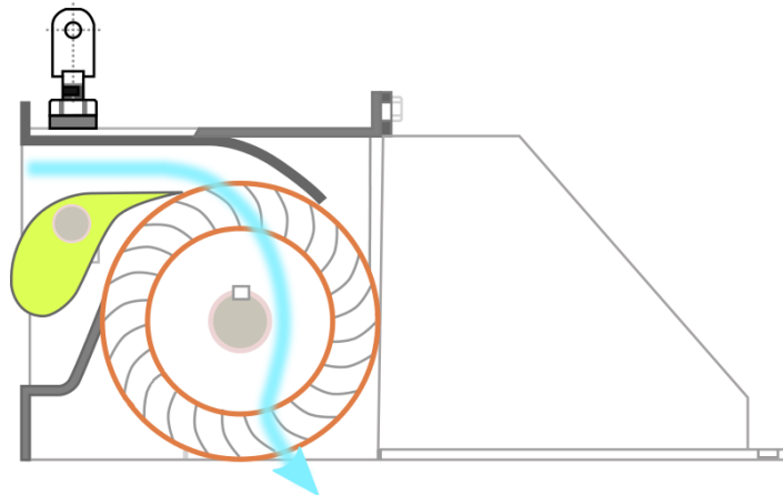
Obr. 1.16: Bánkiho turbína [22]
