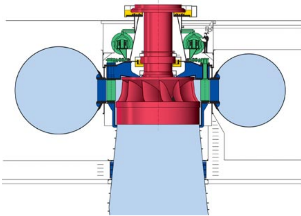
Obr. 1.13: Francisova turbína [19]
