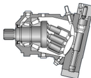
Obr. 22 Hydromotor Bosch Rexroth A6/VM
