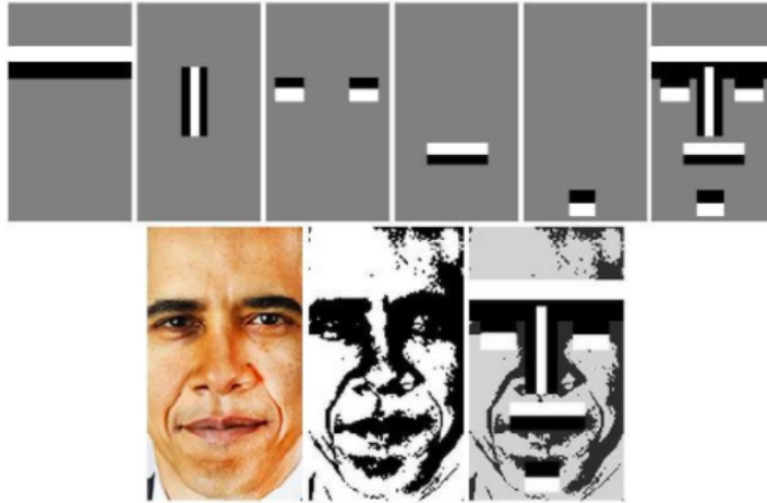
Figure 3.6: Applying the Haar-like feautre types on a face [29]
