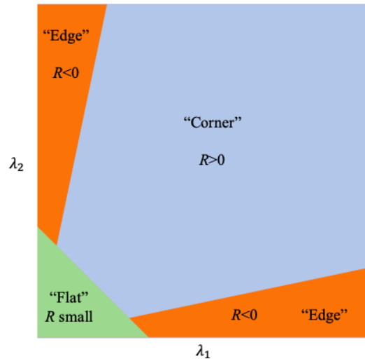
Figure 2.8: Harris measure
