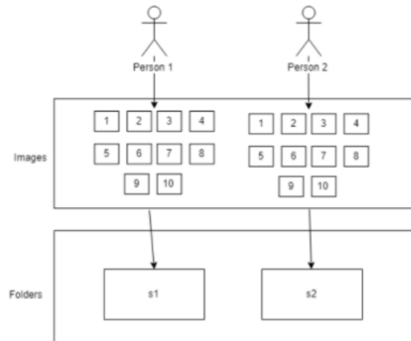
Figure 5.3: Preparing Dataset
