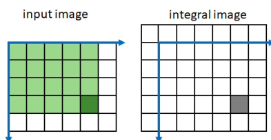
Figure 3.9: Integral Image
