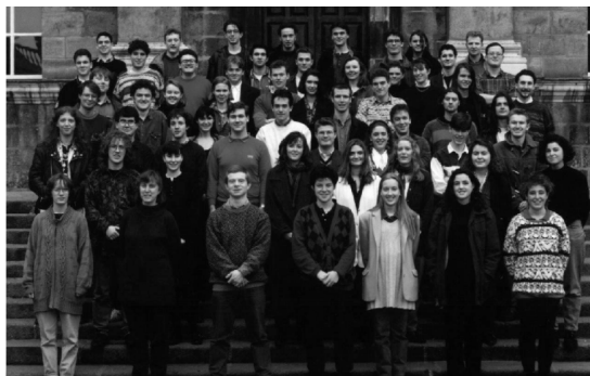
Figure 3.2: Input Image[27]
