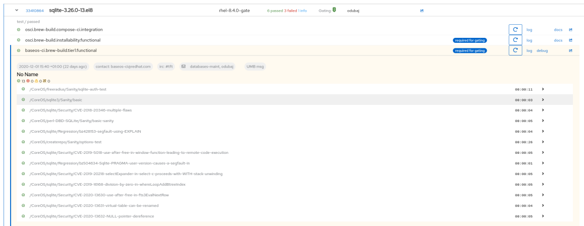
Obr. 5.1: CI Dashboard
