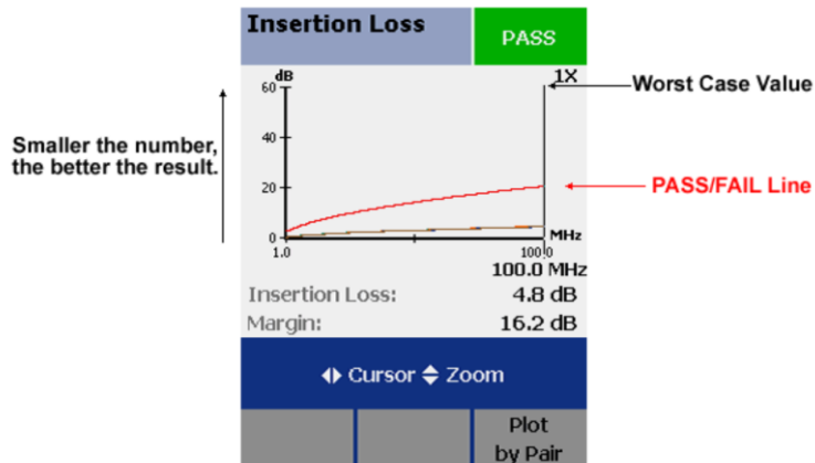
Figure 27 Insertion loss test (Fluke Network, 2021)
