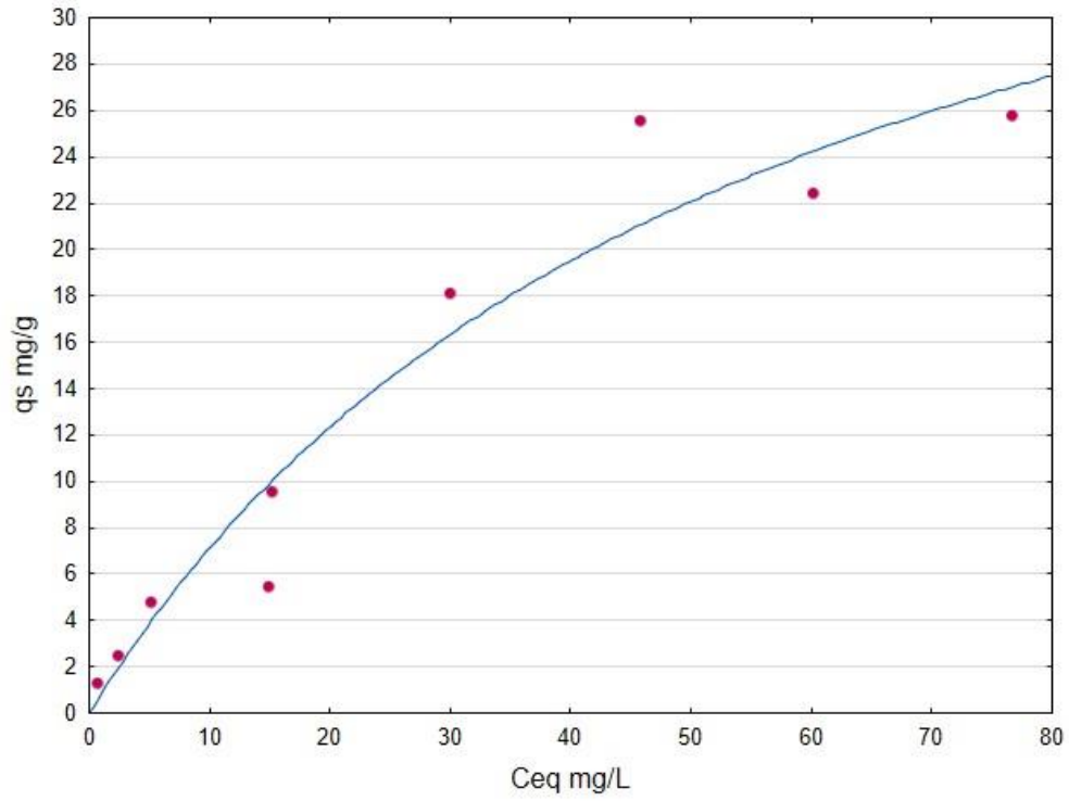
Fig. A19 BTR - BCHTH Langmuir non-linear isotherm
