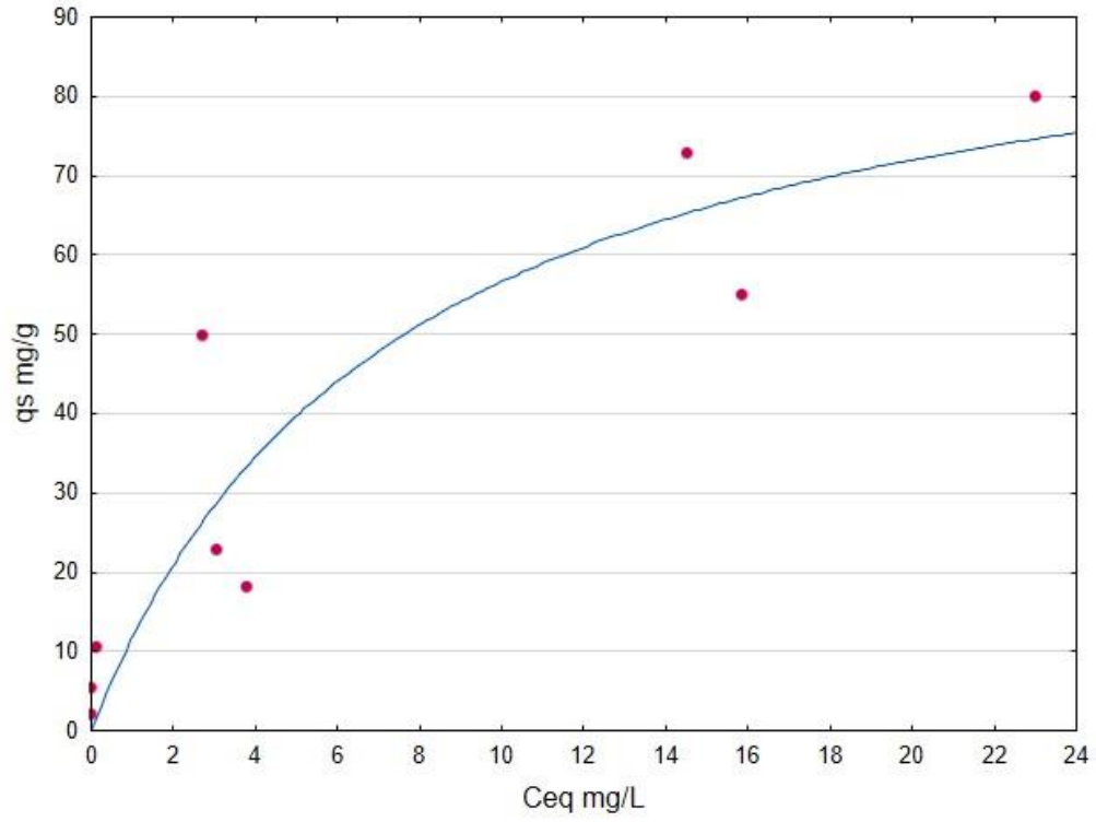
Fig. A23 BTR - BCHSH Langmuir non-linear isotherm
