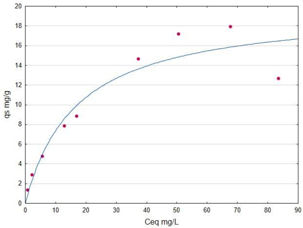
Fig. A9 MTP - BCHTL Langmuir non-linear isotherm
