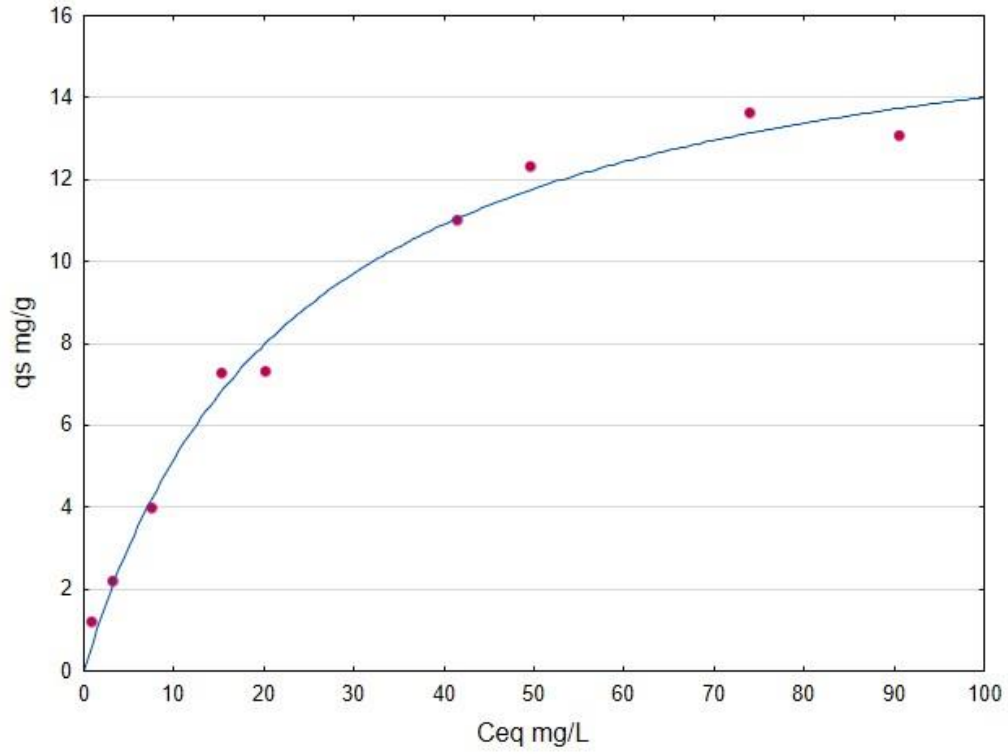
Fig. A17 BTR - BCHTL Langmuir non-linear isotherm
