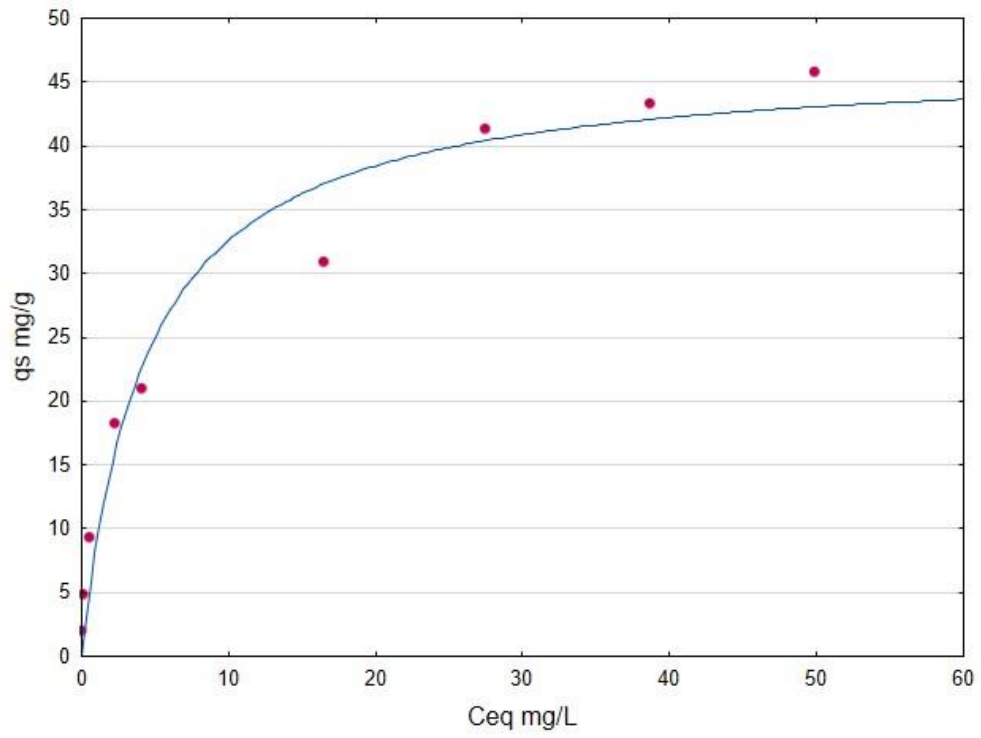
Fig. A13 MTP - BCHSL Langmuir non-linear isotherm
