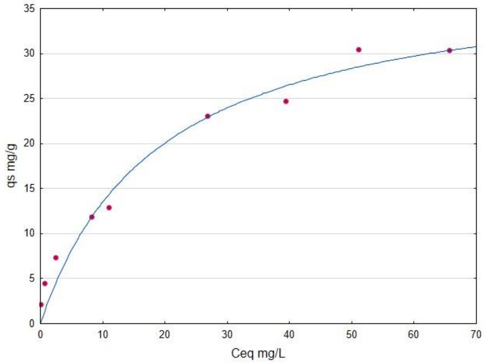
Fig. A11 MTP - BCHTH Langmuir non-linear isotherm
