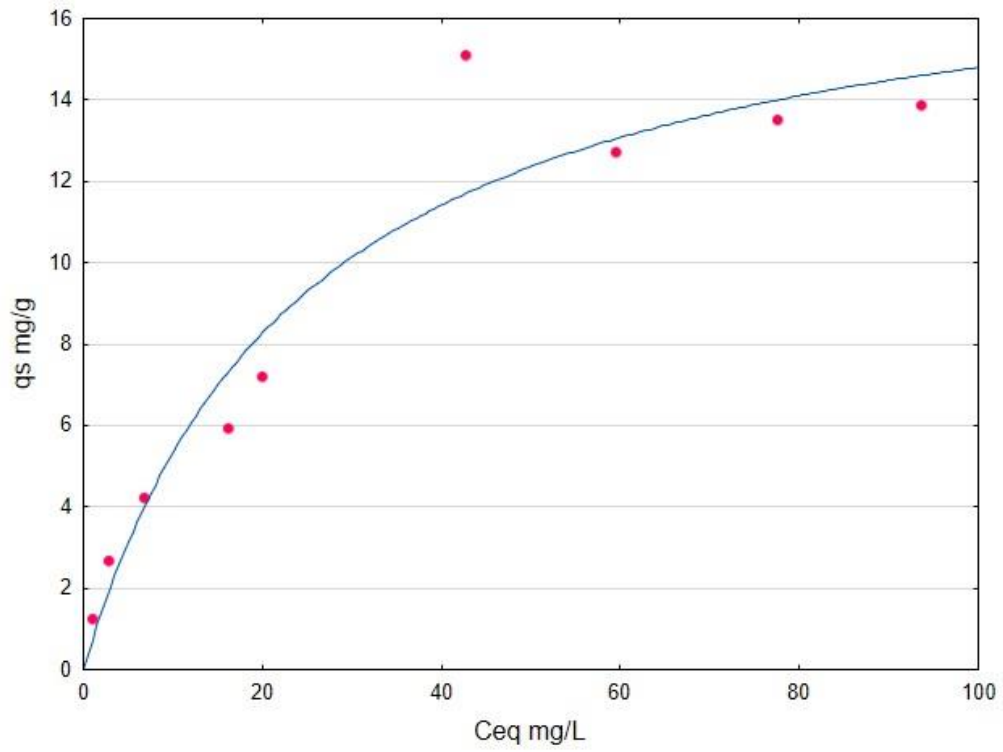
Fig. A3 DCF - BCHTH Langmuir non-linear isotherm
