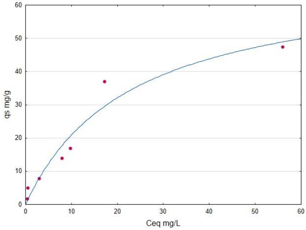
Fig. A21 BTR - BCHSL Langmuir non-linear isotherm
