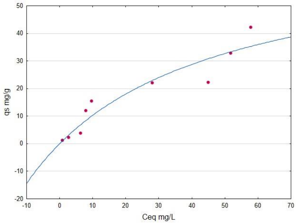
Fig. A5 DCF - BCHSL Langmuir non-linear isotherm
