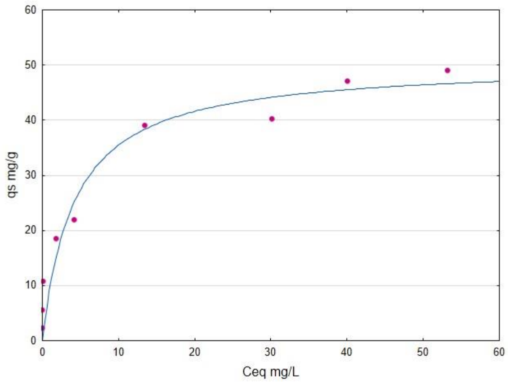
Fig. A7 DCF - BCHSH Langmuir non-linear isotherm
