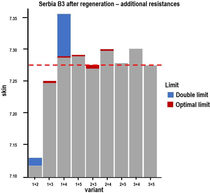
Figure 6. Resulting values of the parameter additional resistances.
