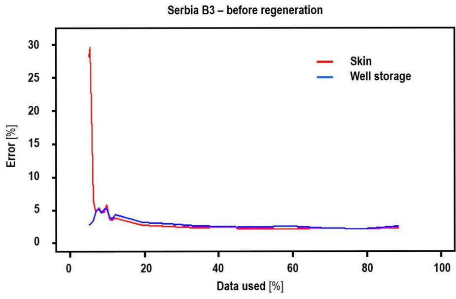
Figure 3. Plot depicting the percentage error for the skin effect and well storage parameters for the well Serbia B3 before regeneration dependent upon the percentage of data used from the pumping test.
