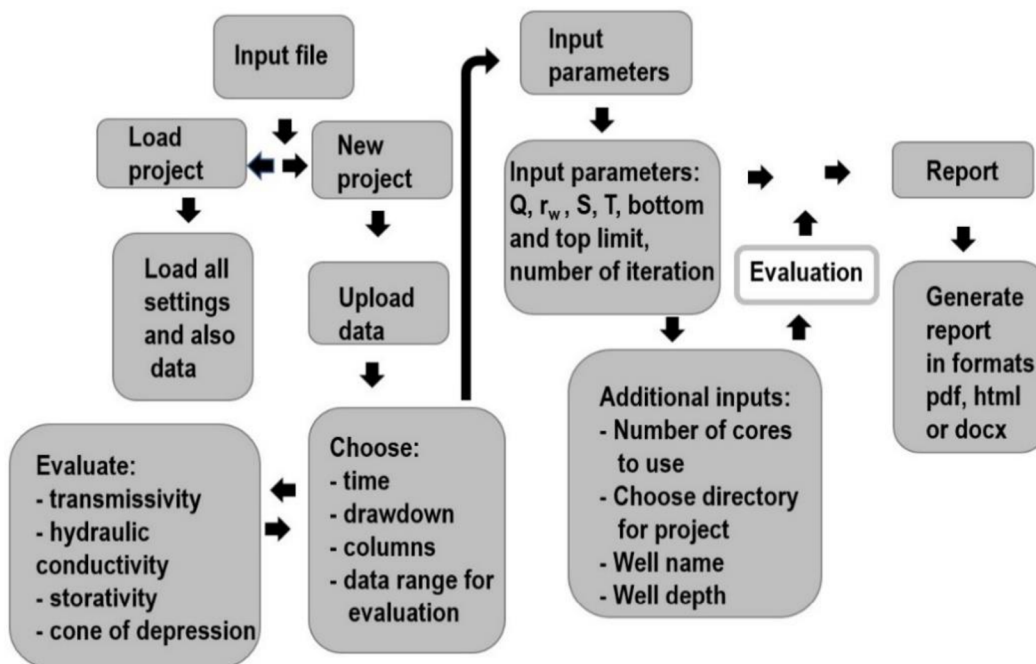
Figure 8. Software diagram.
