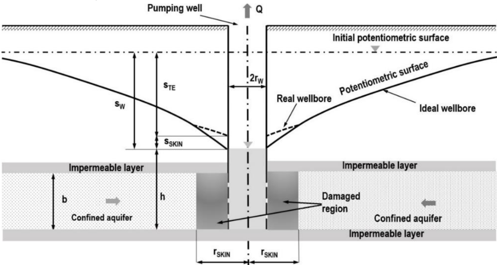
Figure 2. Diagram of a real well: an aquifer stratum with saturated water level.
