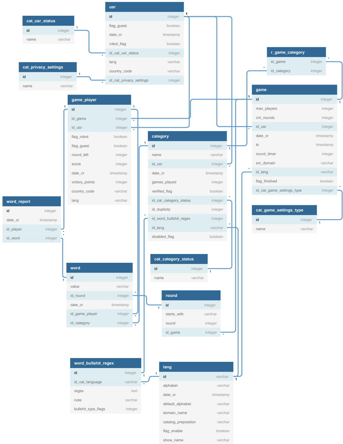
Figure 3.1: Entity relationship diagram of the game database.
