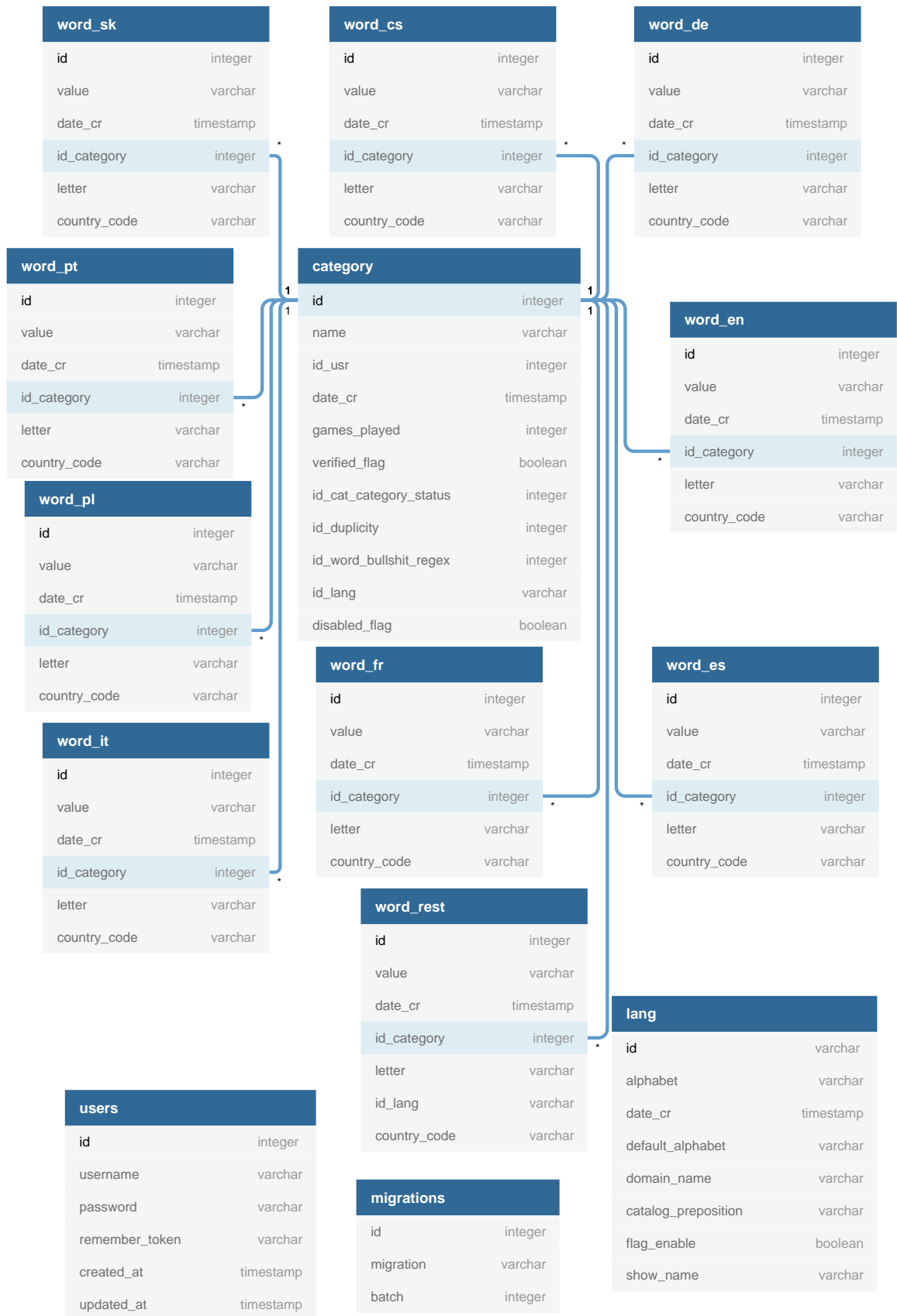
Figure 6.3: Entity relationship diagram of the application database.
