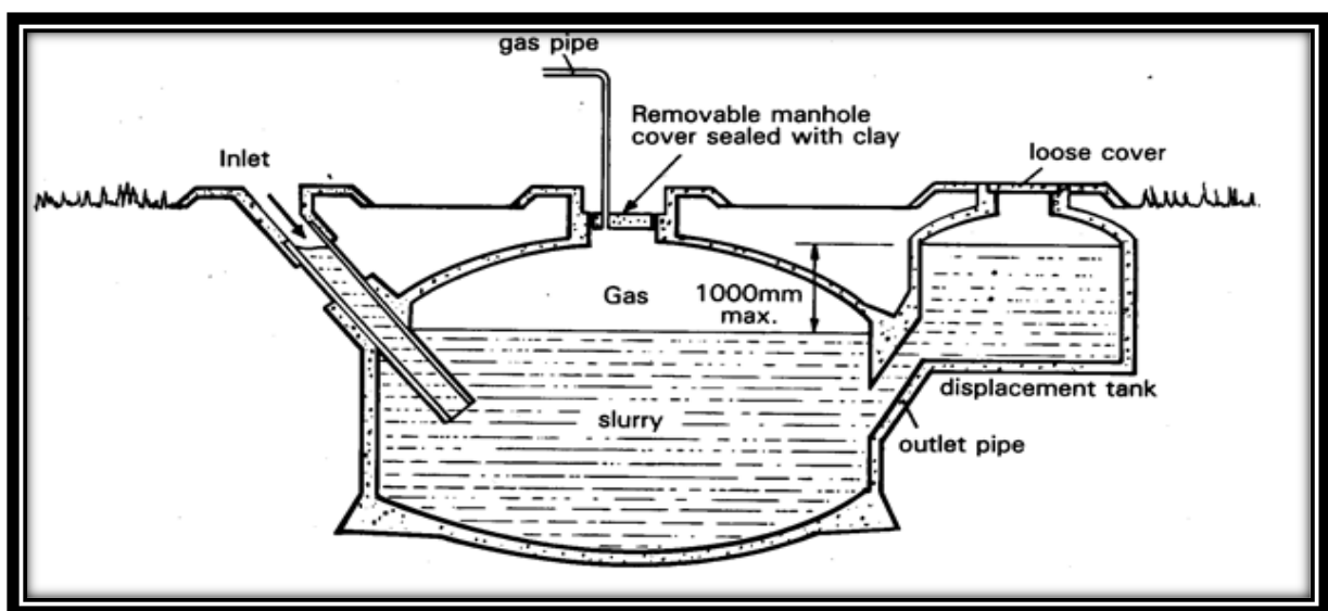
Figure 3: Fixed Dome, Source: (Bansah et al, 2010)
