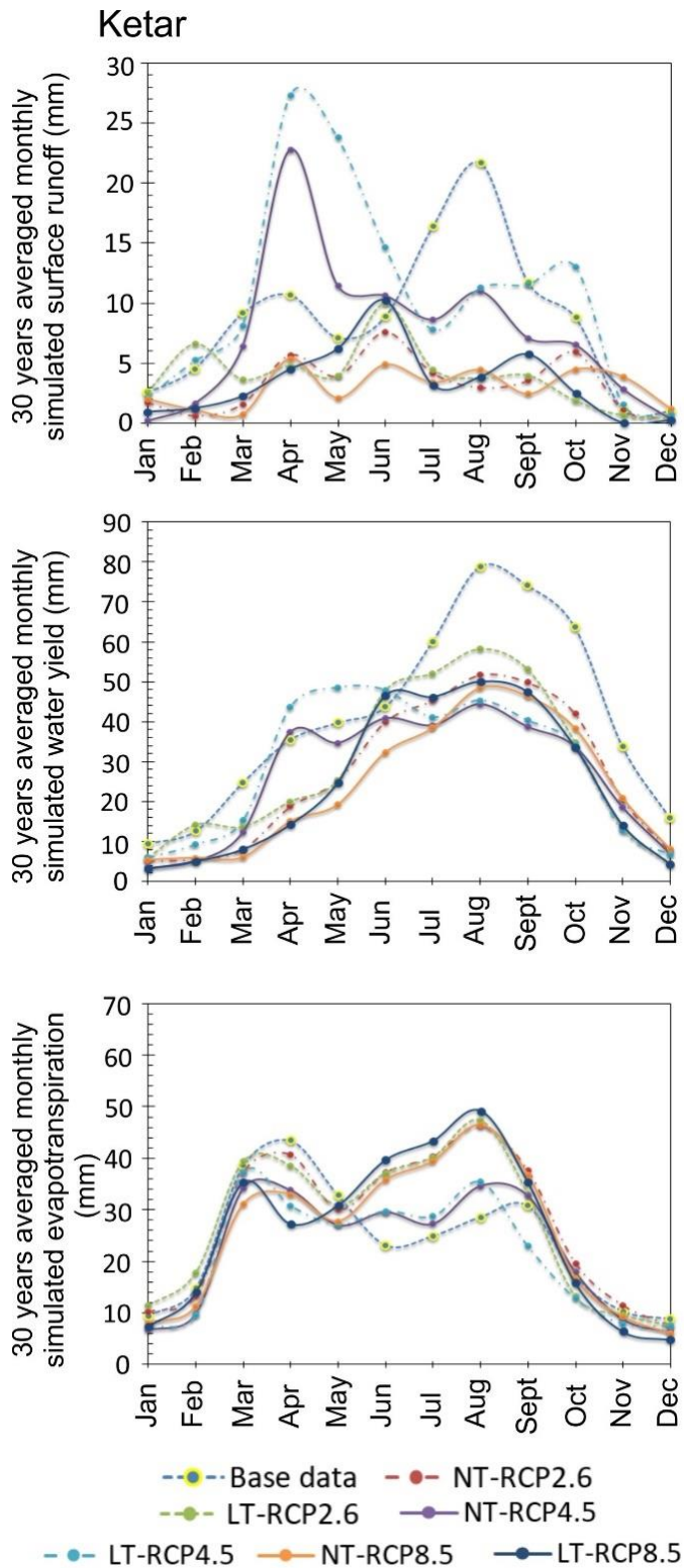
Fig. 9. The simulated monthly distributions of surface runoff, water yield and evapotranspiration in the Ketar sub-basin for the applied scenarios.
