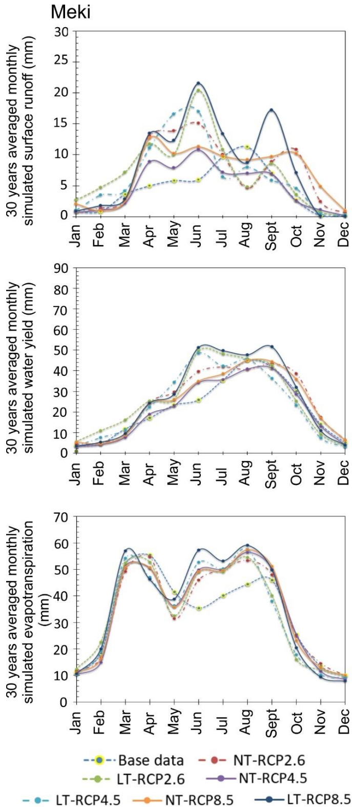
Fig. 10. The simulated monthly distributions of surface runoff, water yield and evapotranspiration in the Meki sub-basin for the applied scenarios.
