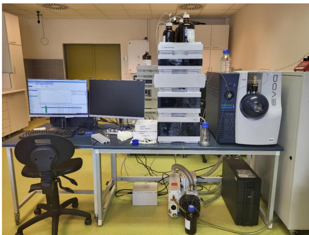
Figure 22: Ultra-High-Performance Liquid Chromatography (UHPLC) Agilent 1290 Infinity with Luna ® Omega Polar C18 column connected with BRUKER EVOQ LC-TQ Mass spectrometer.
