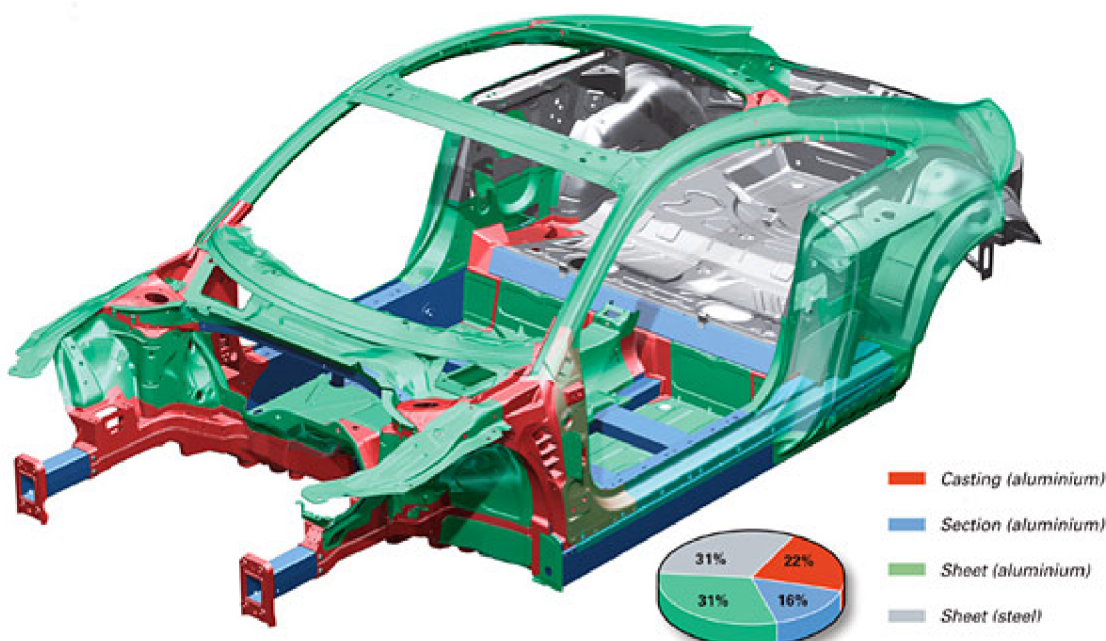
Obr. 14 Audi space frame u vozu Audi TT [14]
