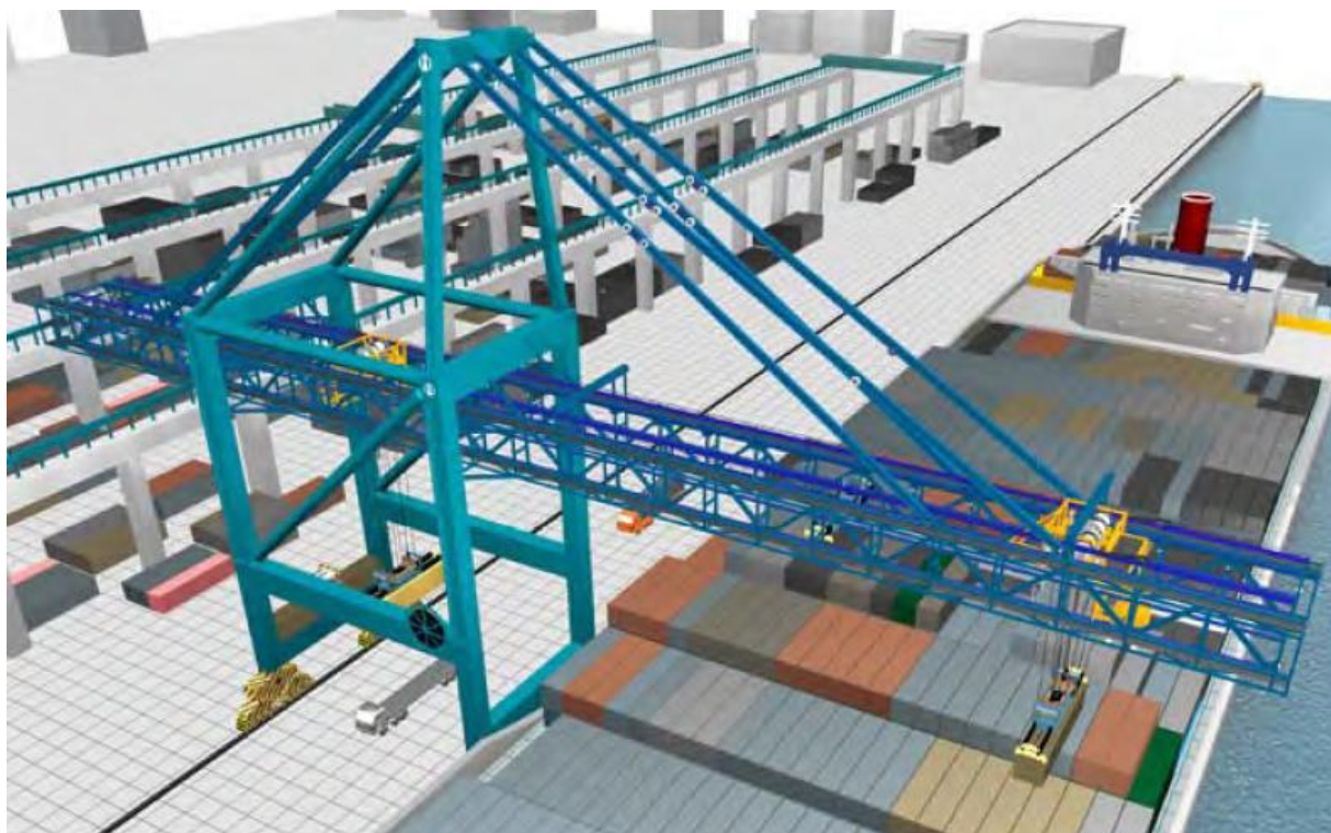
Obr. 32 CreaTech Technotainer [13]
