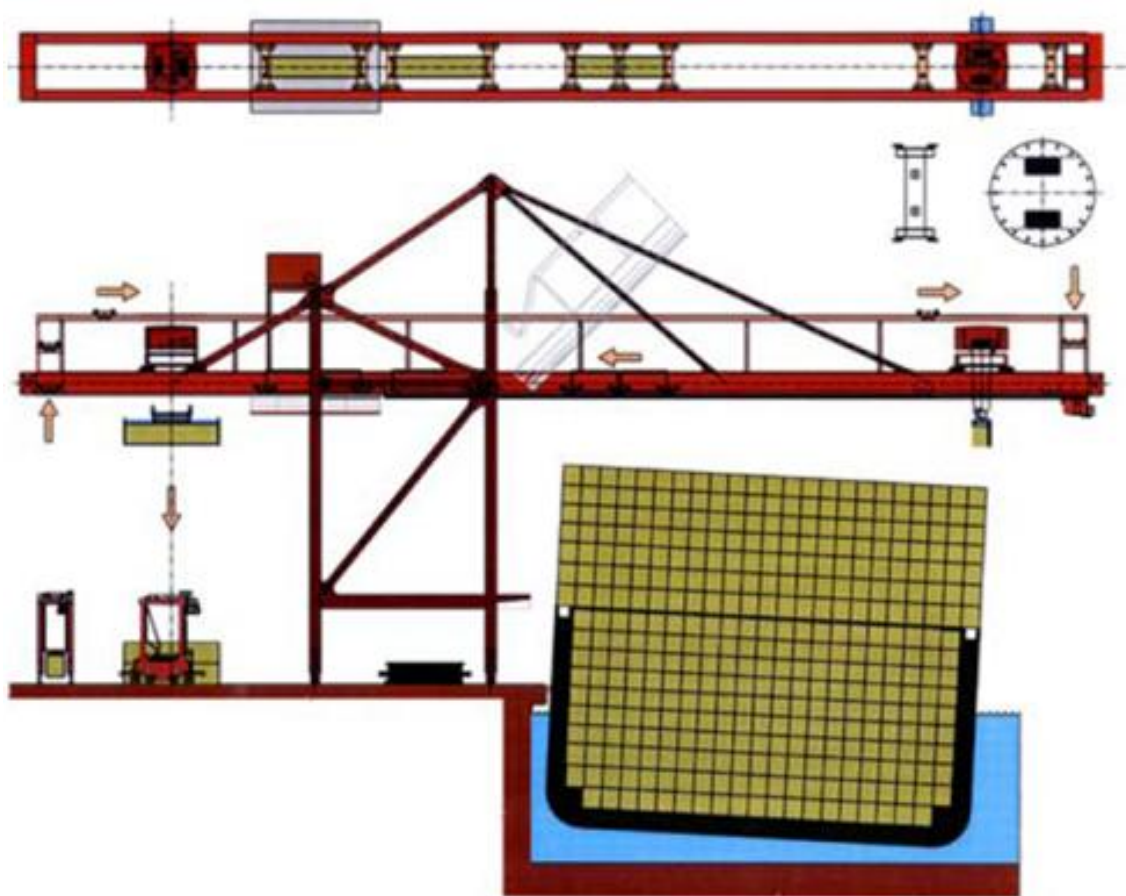
Obr. 34 Liftech SuperCrane [13]
