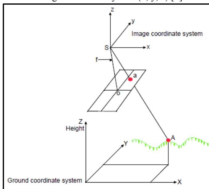
Figure 10 Image space coordinate system [8]
