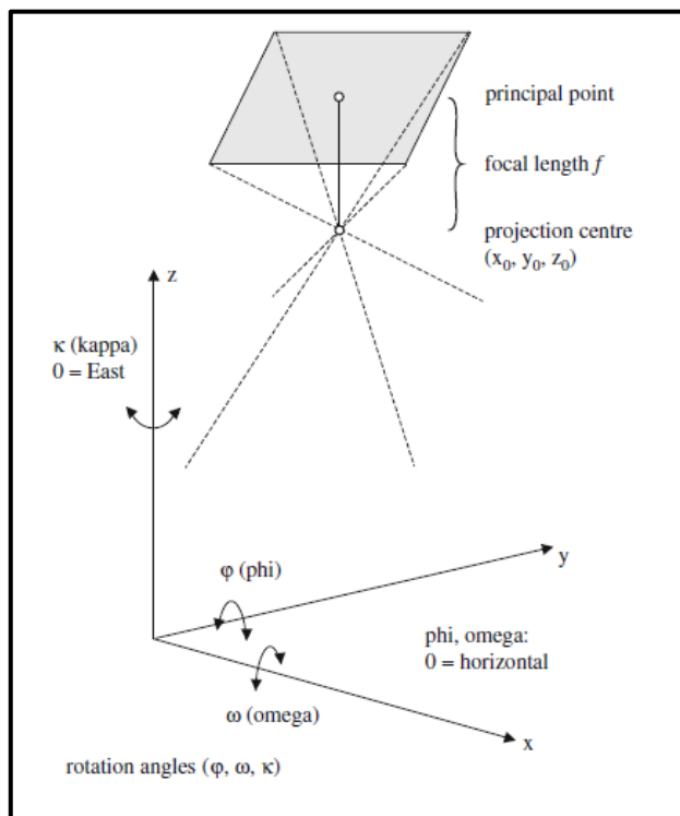
Figure 5 Focal Length, rotation angles and projection centres [4]
