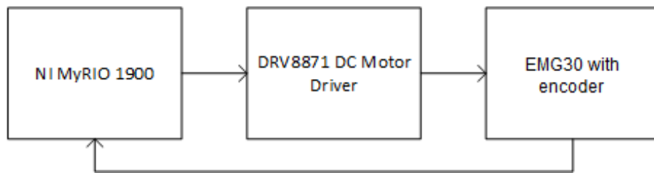
Figure 2.10: HW realization of the positioning feedback loop.
