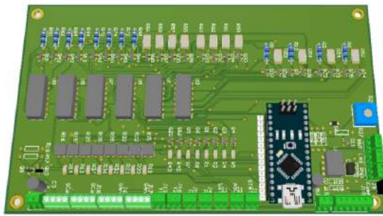
Figure 2.22: Simulated appearance of the control board.
