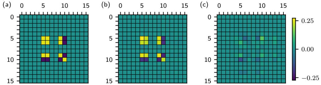
Figure 4.10: Theoretical and experimental density matrix of a four-qubit state produced from input state |\Psi^+\rangle|\Psi^+\rangle by the linear optical quantum gate W . The real part of the theoretical density matrix is shown in panel (a), its imaginary part is zero. Panels (b) and (c) contain the real and imaginary parts of the experimentally reconstructed density matrix, respectively. All the nonzero density matrix elements of \rho_{\text{th}} have absolute value 0.25 and the maximum difference between matrix elements of \rho_{\text{th}} and \rho_{\text{exp}} reads \max_{jk} \Delta\rho_{jk} = 0.149 . The color bar is shared by all matrix plots.
