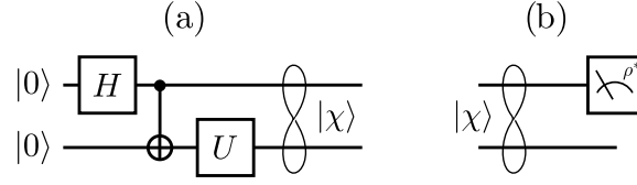
Figure 3.5: Experimental interpretation of Choi's formalism. a) Preparation of |\chi\rangle . The CNOT gate turns input qubits into the maximally entangled state. b) Output generation. The first subsystem of |\chi\rangle is projected to \rho^* , the phase-conjugated input state.
