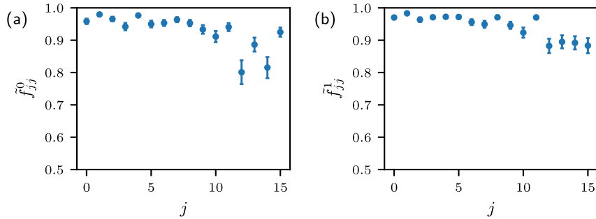
Figure 4.6: Experimental output state fidelities f_{jj}^m for input states forming two mutually unbiased bases. Each input state is a product state with two qubits prepared in the computational basis states and the other two qubits prepared in the superposition states |\pm\rangle . In panel (a), the qubits 1 and 2 were prepared in the superposition |\pm\rangle , while in panel (b) the qubits 3 and 4 were prepared in superposition.
