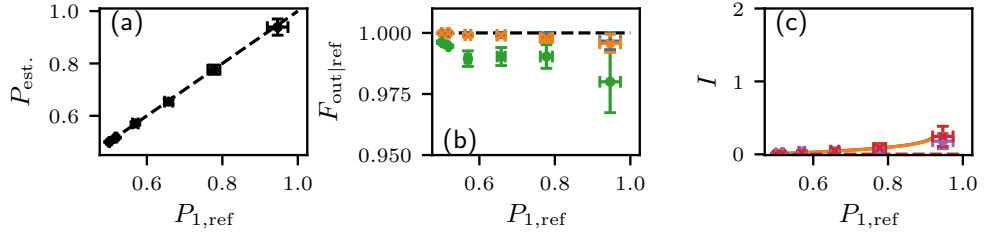
Figure 6.12: Data for the nondemolition measurement of purity using the NDES with error bars corresponding to one standard deviation. The shared horizontal axis shows the purity of a first reference target qubit P_{1,\text{ref}} estimated from state reconstructions with the NDES off. It estimates the input purity. Dashed lines correspond to ideal theoretical predictions, while the points represent the experimental data. Error bars represent one standard deviation calculated over a set of six tested states. (a) Direct nondemolition measurement of purity using NDES. (b) Out-ref-fidelities obtained from tomographic data. Blue and orange color correspond to the first and second target qubit, respectively. Results for joint state target qubits are plotted by green color. (c) Mutual information estimated from the tomographic reconstruction of the target qubits. Purple color represents output state post measurement (NDES on), red colors reference (NDES off). The nearly overlapping solid lines are predictions based on the reconstructed process matrix.
