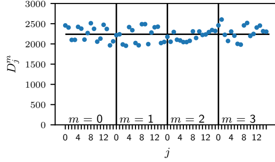
Figure 4.5: The total number of detected two-photon coincidences D_j^m is plotted for the 64 input states |\psi_j^m\rangle , which were utilized in the determination of the truth tables of the four-qubit Toffoli gates in Fig. 4.4.
