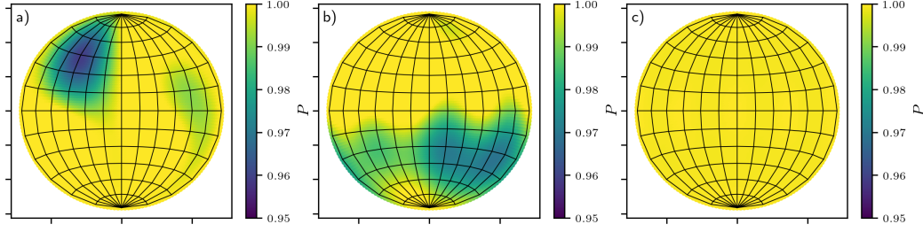
Figure 3.24: State-dependent purity drop artifact. Purity is represented with color. Input states are represented as points on the Bloch sphere in Hammer projection. a) Uncorrected waveplate imperfection ( \delta\Gamma_1 = \delta\Gamma_2 = -3 deg), ideal projections are assumed in reconstruction. The typical purity drop area appears. b) True projectors are known and taken into account in reconstruction, but the renormalization of projectors is not performed. c) True projectors and known and taken into account in reconstruction along with proper renormalization.
