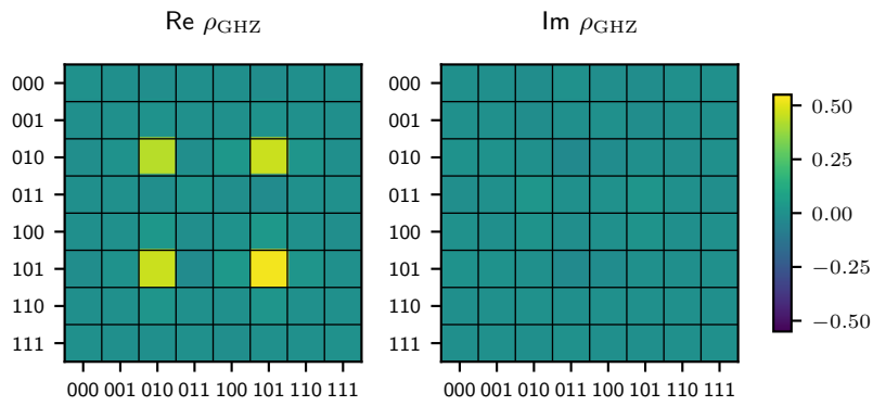
Figure 6.9: The matrix plot of the GHZ-like state prepared by the Fredkin gate.
