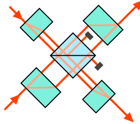
Figure 3.21: Crossed MZIs sharing a PPBS. Only photons propagating through the nondisplaced paths interfere at the central PPBS. We depicted the undetected reflections from PPBS with dark beam stops.
