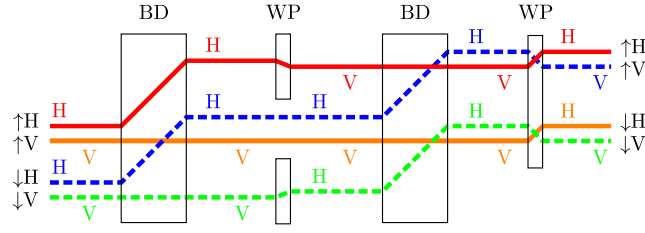
Figure 6.3: An illustrative scheme depicting the essence of our SWAP gate implementation for two photonic qubits encoded in path and polarization modes of a single photon. The different optical modes are denoted by the different colors and line styles to distinguish them.
