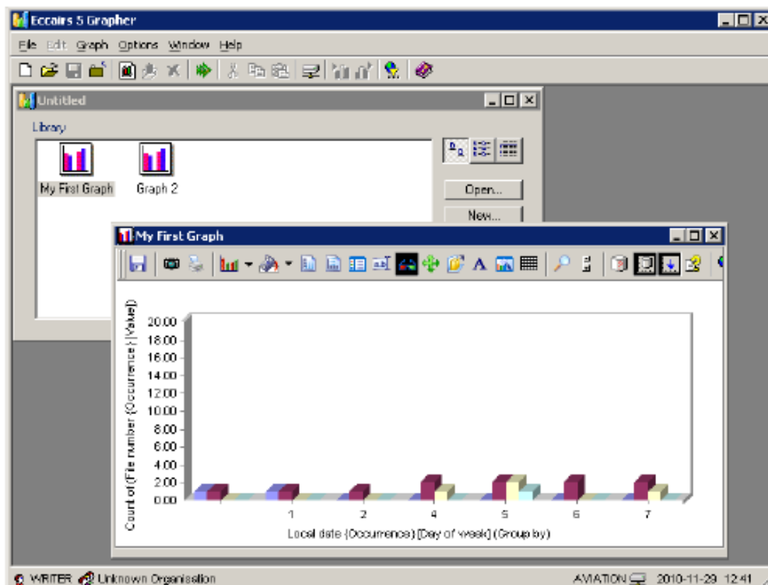
Obr. 2.12: ECCAIRS Grapher [4]
