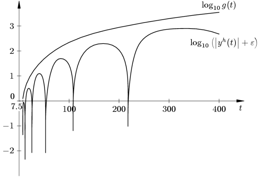
Fig. 6.1: The solution \log_{10}(|y^h(t)| + \epsilon) and its estimate.
