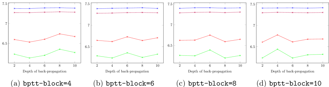
Figure 4.2: Comparison of simple recurrent network (SRN) performance with respect to how often a weights update is performed. Green is the error obtained while training; red is the error on the training dataset obtained with fixed weights; blue and purple are validation and test errors respectively.
