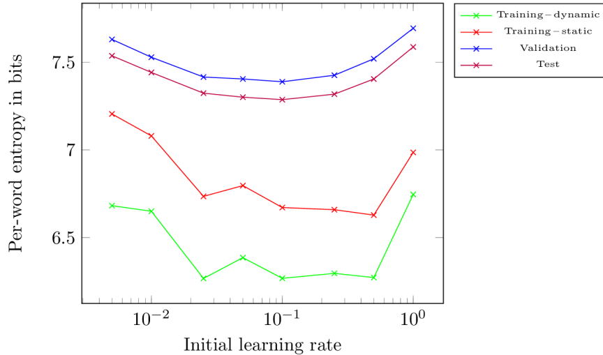
Figure 4.3: Performance of a simple recurrent network (SRN) with respect to the initial learning rate. Results are average of 3 networks with different random initialization. The rough results for training set can be simply explained by effects of the random initialization and noise in the training data.
