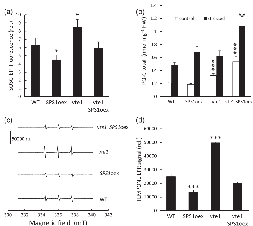
FIGURE 4 ^1\text{O}_2 scavenging by plastoquinone-9. (a) ^1\text{O}_2 production by leaves in the light as measured by SOSG-EP fluorescence. Attached leaves were infiltrated with SOSG and exposed for 20 min to light ( 1,500 \mu\text{mol photons m}^{-2} \text{s}^{-1} ) at 7^\circ\text{C} . Data are mean values of minimum four measurements. (b) Total PQ-C levels in leaves before and after high light stress ( 1,500 \mu\text{mol photons m}^{-2} \text{s}^{-1} for 2 days at 7^\circ\text{C} ). Data are mean values (in nmoles per mg leaf fresh weight) of three separate measurements \pm SD. (c-d) ^1\text{O}_2 production by thylakoids as measured by the spin probe TEMPONE and EPR spectroscopy. No signal was detected in the dark. (c) TEMPONE EPR traces and (d) quantification of the TEMPONE EPR signal. Data are mean values of three separate measurements \pm SD. *, **, and ***, different from WT at p < .01 , .005 , and .001 (Student's t test). ^1\text{O}_2 = singlet oxygen; SOSG = singlet oxygen sensor green; EP = endoperoxide; PQ-C = Hydroxyplastoquinone; F.W. = fresh weight; TEMPONE = 2,2,6,6-tetramethyl-4-piperidone-1-oxyl; EPR = electron paramagnetic resonance
