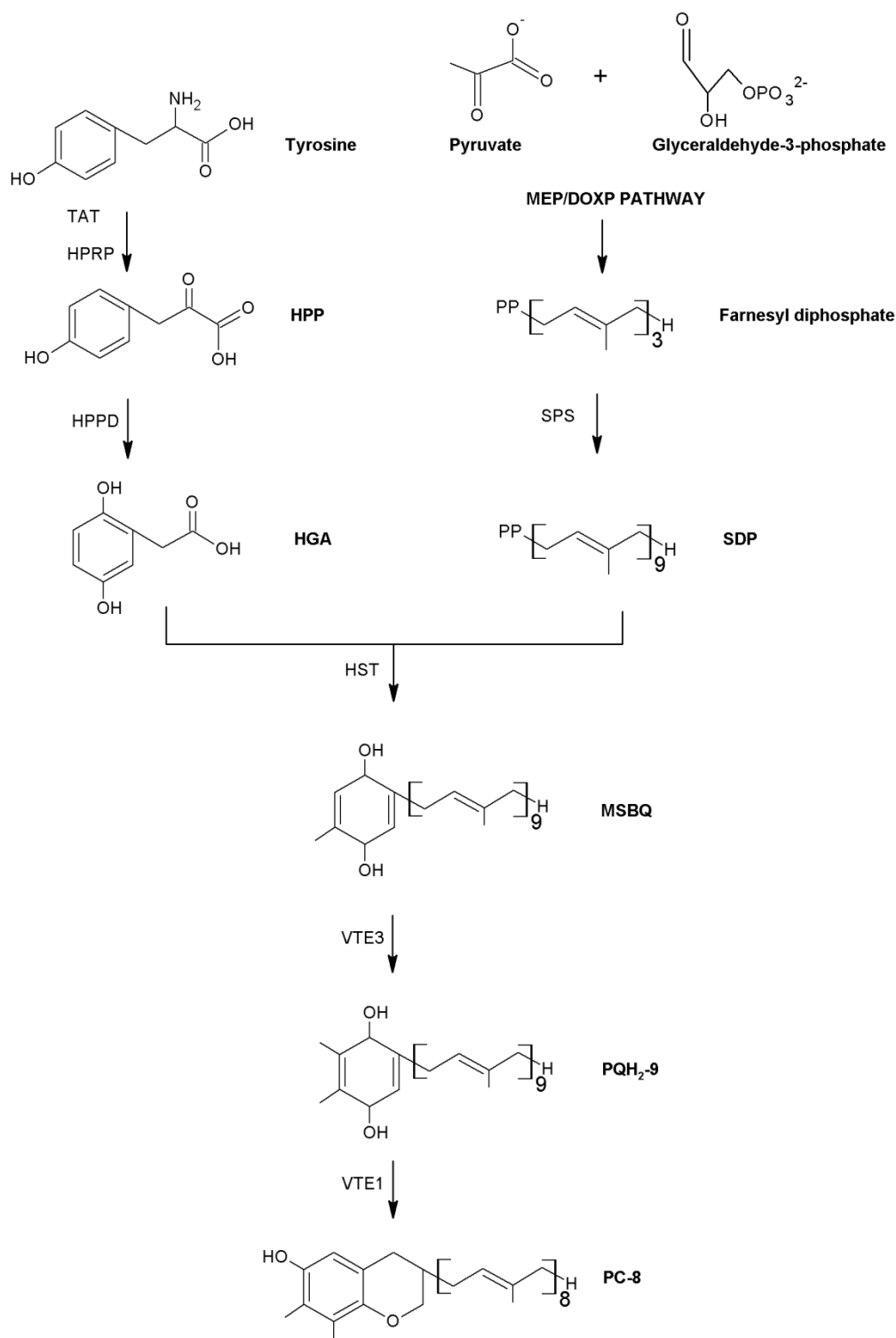
Figure 10. Plastoquinone-9 and plastochromanol-8 biosynthetic pathway. TAT, tyrosine aminotransferase; HPRP, 4-hydroxyphenylpyruvate reductase; HPPD, 4-hydroxyphenylpyruvate dioxygenase; HGA, homogentisic acid; MEP/DOXP pathway, methylerythritol 4-phosphate/deoxy-d-xylulose-5-phosphate; SPS, solanesyl diphosphate synthase; SDP, solanesyl diphosphate; HST, homogentisate solanesyl transferase; MSBQ, 2,3-dimethyl-6-solanesyl-1,4-benzoquinol, VTE3, phytylbenzoquinone methyltransferase; VTE1, tocopherol cyclase. Scheme created by modifications from (Nowicka and Kruk, 2010; Havaux, 2020).
