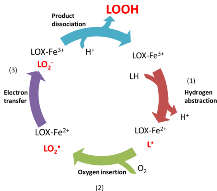
Figure 17. Lipoxigenase reaction mechanism. In reaction (1), the hydrogen is abstracted from unsaturated fatty acids (LH) by the active site of enzyme (LOX-Fe 3+ ) forming L • , while the electron from carbon-hydrogen bond reduces ferric to ferrous non-heme iron, while proton is stored for following protonation (LOX-Fe 2+ ). In reaction (2), the addition of 3 O 2 to L • leads to LO 2 • . In reaction (3), ferrous non-heme iron oxidizes to ferric non-heme iron, while protonates LO 2 • to LOOH. Modified by Brash, 1999.
