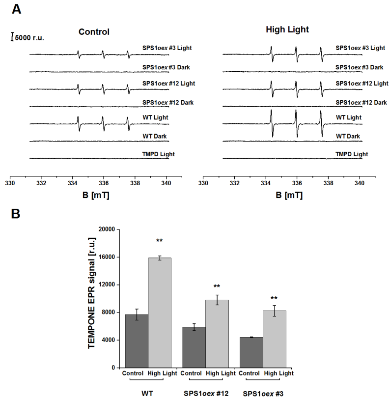
Figure 3. Singlet oxygen formation in broken chloroplasts of control and high light exposed WT and SPS1oex Arabidopsis plants detected by EPR spin-trapping spectroscopy. (A) TEMPONE EPR spectra detected after 30 min white light treatment ( 1000 \mu\text{mol photons m}^{-2} \text{s}^{-1} ) of broken chloroplasts from Arabidopsis in the presence of 50 mM TMPD. TEMPONE EPR spectrum of pure probe (bottom spectrum) was obtained after illumination of 50 mM TMPD and 40 mM MES-NaOH buffer (pH 6.5) with white light ( 1000 \mu\text{mol photons m}^{-2} \text{s}^{-1} ) for 30 min. (B) The intensity of TEMPONE EPR signal was determined by measuring the relative height of central peak of the EPR absorption spectrum. Presented data are mean values ( n = 3 ), \pm SD. The asterisk indicates significant difference between control and high light exposed WT and SPS1oex Arabidopsis (Student's test). Significant differences were confirmed also between WT and SPS1oex Arabidopsis (ANOVA).
