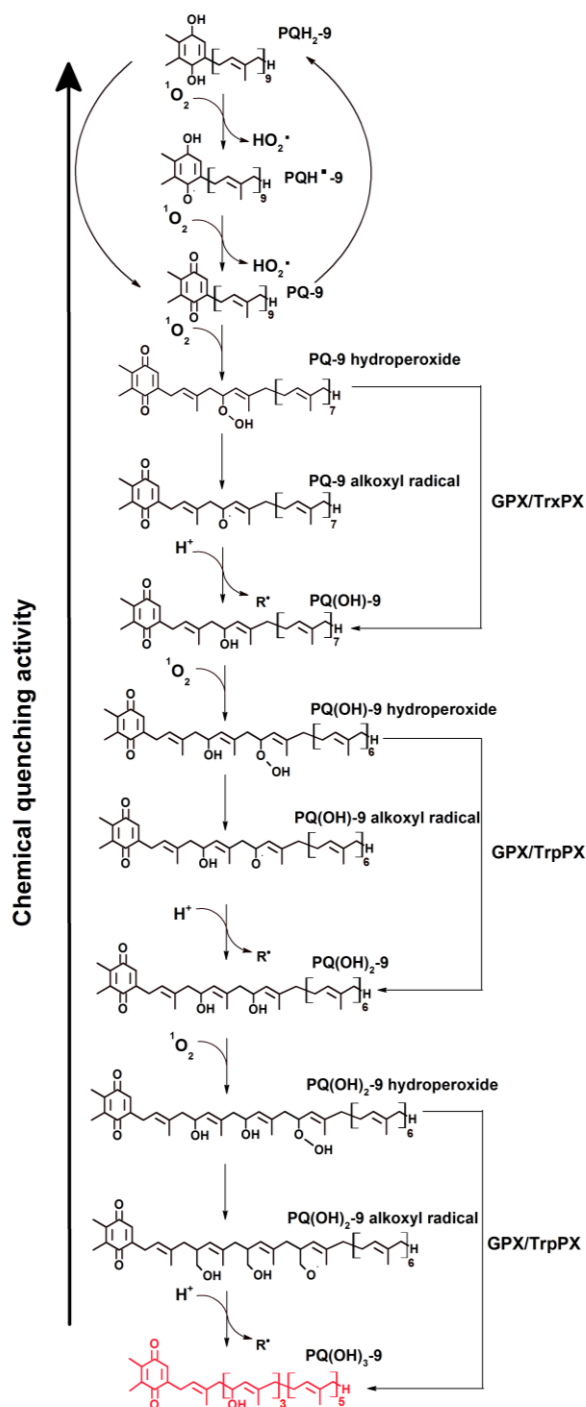
Figure 15. Formation of trihydroxyplastoquinone-9. Plastoquinol-9 function as an antioxidant of ^1\text{O}_2 is illustrated. After \text{PQH}_2\text{-9} oxidation with ^1\text{O}_2 the well-known product \text{PQ-9} is formed via \text{PQH}^\bullet\text{-9} , producing two molecules of \text{HO}_2^\bullet which dismutate into \text{H}_2\text{O}_2 . Subsequently reaction of \text{PQ-9} with another ^1\text{O}_2 molecule produces \text{PQ(OH)-9} through decomposition of \text{PQ-9} hydroperoxide by 1) radical reaction pathway comprising of \text{PQ-9} alkoxy radical as intermediate or 2) non-radical reaction pathway caused by enzymes of the glutathione peroxidase (GPX) or thioredoxin peroxidase (TrxPX) families. Oxidation of \text{PQ(OH)-9} probably proceeds similarly through \text{PQ(OH)-9} hydroperoxide formation and decomposition by a radical or non-radical reaction to \text{PQ(OH)}_2\text{-9} , from which \text{PQ(OH)}_3\text{-9} is produced via \text{PQ(OH)}_2\text{-9} hydroperoxide in the same way.
