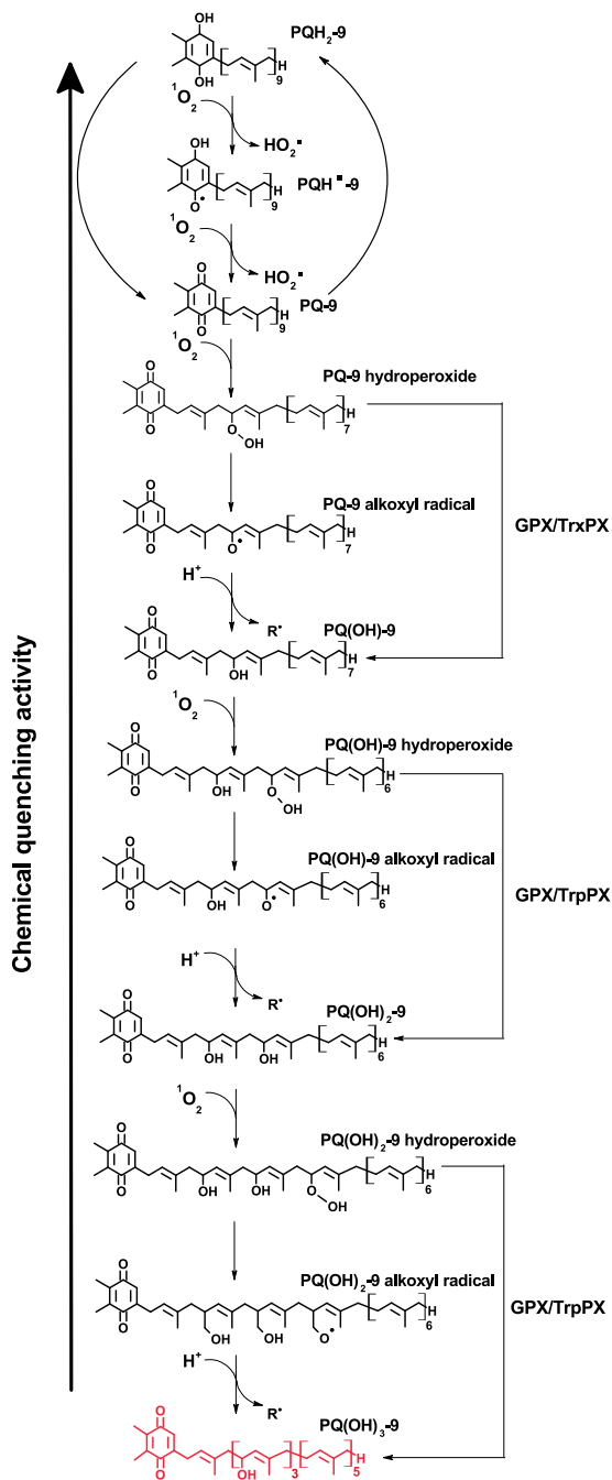
Figure 8. Formation of trihydroxyplastoquinone-9 [PQ(OH) 3 ]. Plastoquinol-9 (PQH 2 -9) function as an antioxidant of ^1\text{O}_2 is illustrated. After PQH 2 -9 oxidation with ^1\text{O}_2 , a well-known product plastoquinone-9 (PQ-9) via PQH • -9 is formed, producing two molecules of HO 2 • that dismutate into H 2 O 2 . Subsequently, reaction of PQ-9 with another ^1\text{O}_2 leads to hydroxyplastoquinone-9 [PQ(OH)-9] through decomposition of PQ-9 hydroperoxide by: (1) radical reaction pathway comprising of PQ-9 alkoxy radical as intermediate; or (2) non-radical reaction pathway caused by enzymes of the glutathione peroxidase (GPX) or thioredoxin peroxidase (TrxPX) families. Following oxidation of PQ(OH)-9 probably proceeds similarly through PQ(OH)-9 hydroperoxide decomposition by a radical or non-radical reaction to dihydroxyplastoquinone-9 [PQ(OH) 2 -9] from which trihydroxyplastoquinone-9 [PQ(OH) 3 -9] is produced via PQ(OH) 2 -9 hydroperoxide in the same way. [Colour figure can be viewed at wileyonlinelibrary.com ].
