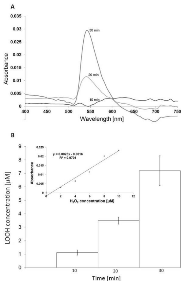
Figure 19. Quantification of hydroperoxide formation in Chlamydomonas cells ferrous oxidation-xylene orange assay. In (A) absorption spectra of FOX reagent with Chlamydomonas cells heated for 10, 20 and 30 min measured in the spectral ranges of 400–750nm. In (B) the concentrations of LOOH was established from the calibration curve with H 2 O 2 as substrate (equation y = 0.0025x - 0.0016 ; shown in the insert) were as follow: 1.12 \pm 0.19 \mu\text{M} (10min), 3.49 \pm 0.26 \mu\text{M} (20min) and 7.19 \pm 1.11 \mu\text{M} (30min). The coefficient of determination R^2 was determined as 0.9701.
