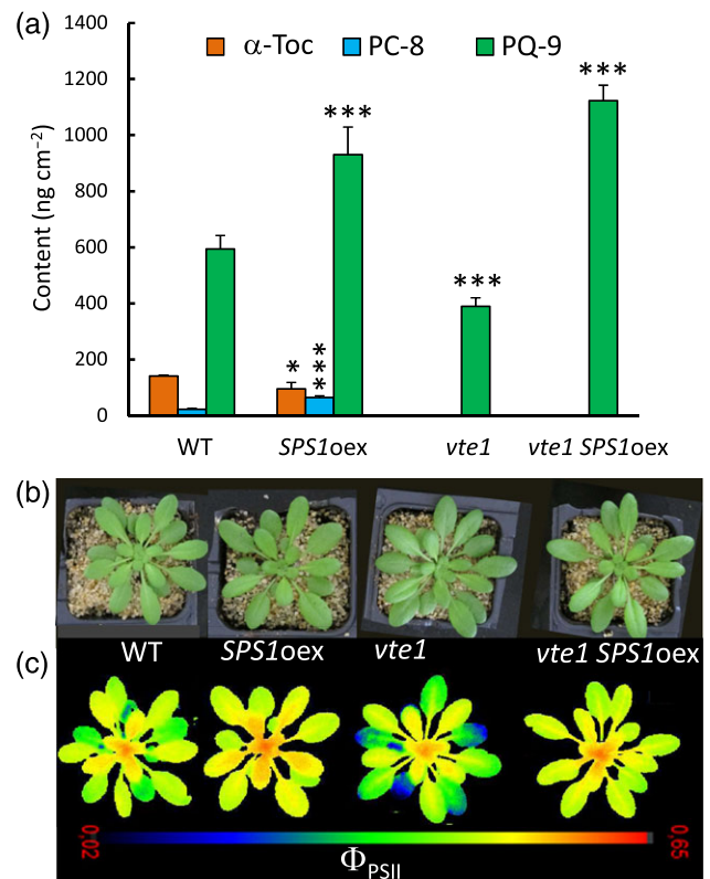
FIGURE 1 Accumulation of PQ-9 in the Arabidopsis vte1 SPS1 oex plants. (a) α-Toc, PC-8, and PQ-9 concentrations in leaves of WT Arabidopsis, the single mutant vte1 , the SPS1 overexpressor SPS1 oex, and the double mutant vte1 SPS1 oex (obtained by crossing vte1 with the SPS1 oex Line #12 previously described in Ksas et al., 2015). Data are mean values of four separate measurements ± SD. (b) Picture of the different genotypes at the age of 4 weeks. (c) Images of the efficiency of PSII-mediated electron transport \Phi_{PSII} in plants illuminated with red light of PFD 230 µmol photons m -2 s -1 . * and ***, different from WT at p < .01 and .001 (Student's t test). PC-8 = plastochromanol-8; PQ-9 = plastoquinone-9; α-Toc = α-tocopherol; PSII = photosystem II
