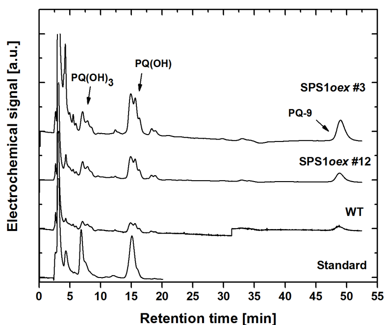
Figure 13. HPLC chromatograms of trihydroxyplastoquinone-9. Standard chromatogram of 10 \mu M PQ-9 in methanol with Rose Bengal as photosensitizer, after 10 min illumination (1500 \mu mol photons m^{-2} s^{-1} ). Chromatograms of high light exposed WT and SPS1oex lines #12 and #3 Arabidopsis in methanol.
