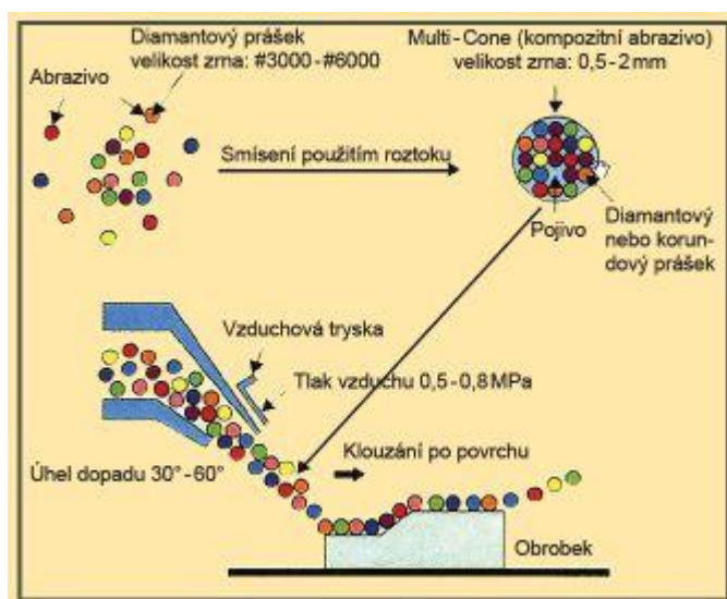
Obr. 21 Mechanismus Multi-Cone [21].
