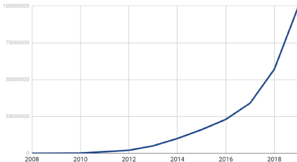
Figure 4.1: Github growth
