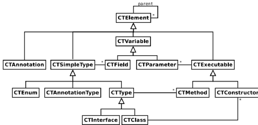
Figure 3.2: Structure of the element.
