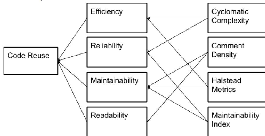
Figure 2.1: Relations between code characteristics and quality metrics.
