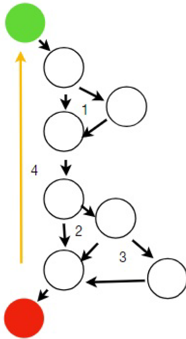
Figure 2.2: Cyclomatic complexity example.
