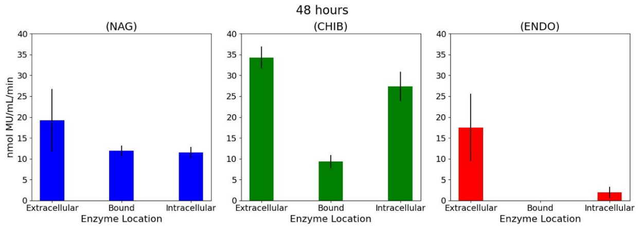
Figure 9: Trial 2 histograms of chitinase activity of extracellular, bound, and intracellular enzymes for 24h and 48h samples. A 24h sample after 15 min of reaction. B 48h sample after 15 min of reaction.
