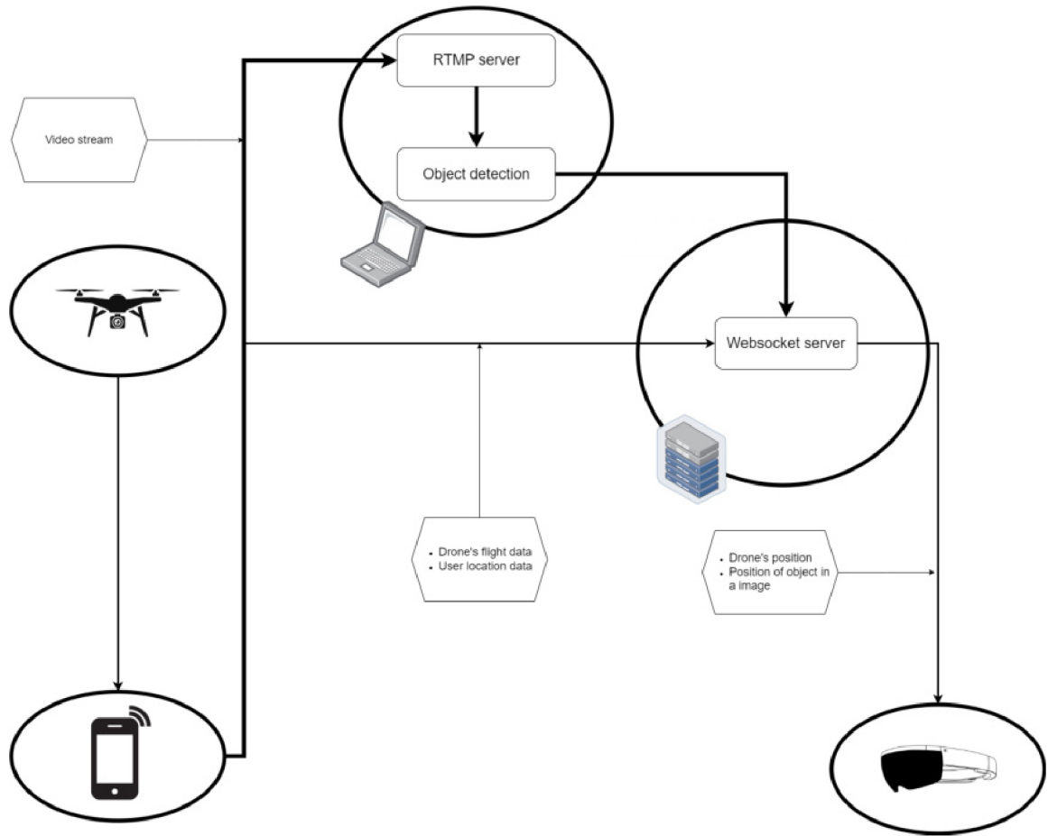
Figure 6.12: Adjusted system overview accounting for limited cellular data bandwidth.
