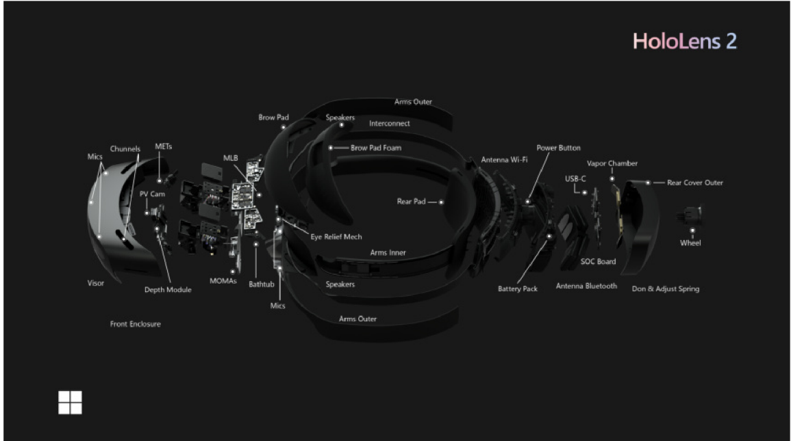
Figure 4.1: Microsoft HoloLens 2 component list. 1
