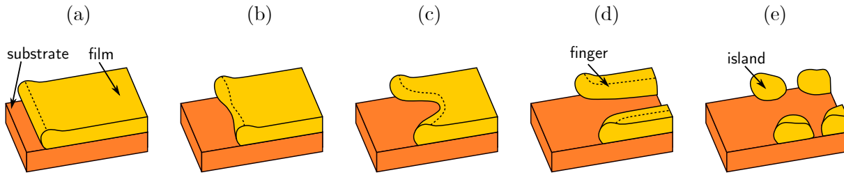
Figure 1.5: Fingering instabilities: (a) rim formation; (b) perturbation development; (c) locally increased edge retraction; (d) finger formation; (e) subsequent island formation due to a Rayleigh-Plateau instability.
