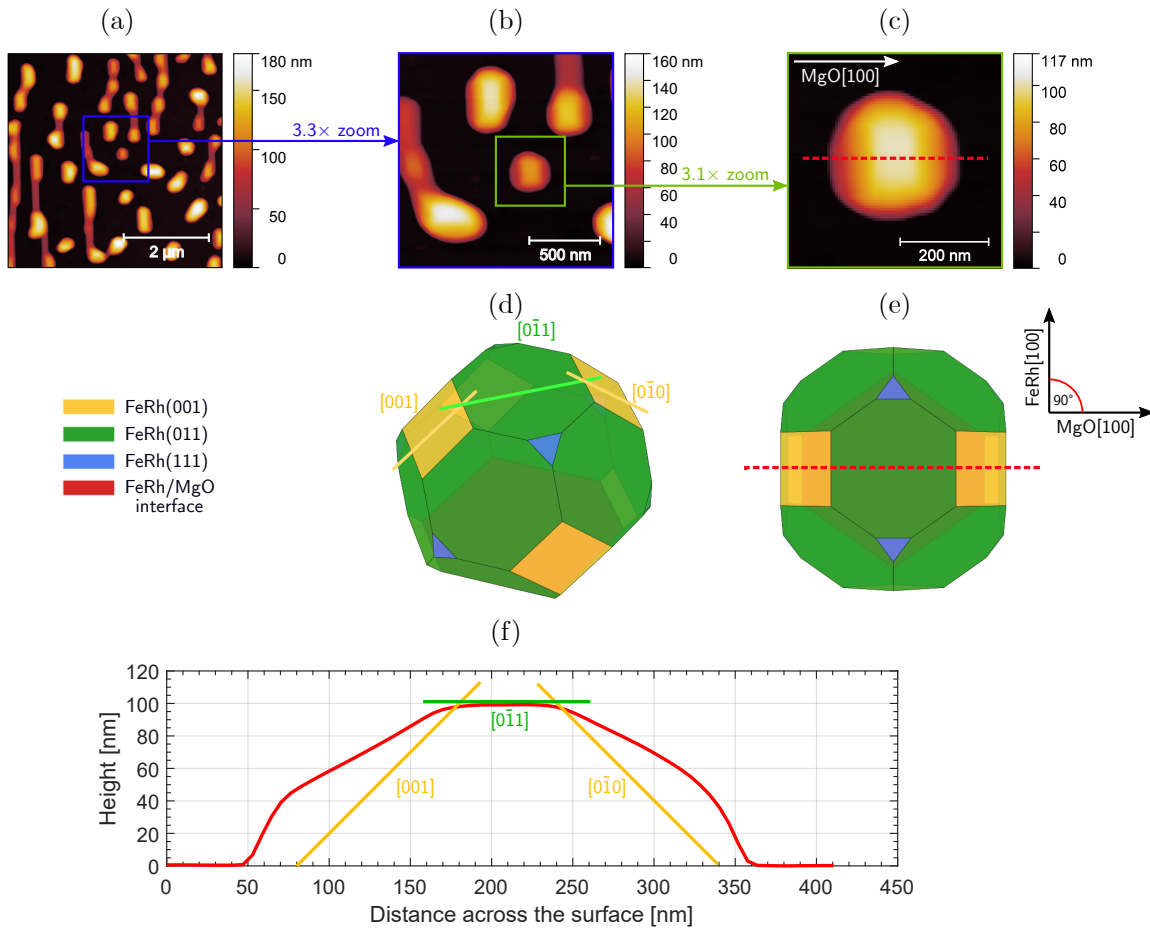
Figure 2.11: Nanoisland shape analysis of FeRh on MgO(011): (a) AFM image of sample M(011)-16; (b) high-resolution image of a 1.5 \times 1.5 \mu\text{m}^2 region from (a); (c) close-up of a 300-nm-wide island from (b). The dashed line indicates the position of the line-scan shown in (f). (d) Oblique view of the FeRh(100)/MgO(011) Winterbottom construction, showing the FeRh lattice directions corresponding to the facet path across the particle as indicated in (e). (e) Top view of the Winterbottom construction, showing a comparable projection of the island shape experimentally observed in (c). (f) Experimental height profile extracted from the line-scan in (c). Superimposed straight lines indicate the facet directions as theoretically extracted from the Winterbottom construction in (d) and (e).
