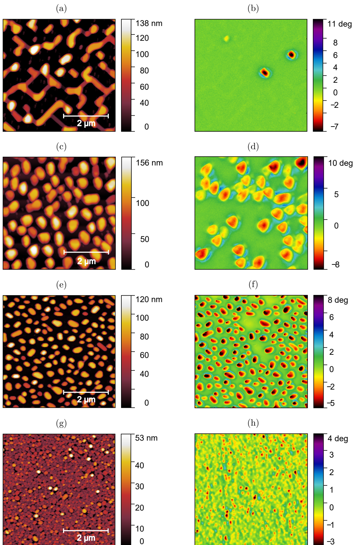
Figure 3.1: AFM (left panel) and MFM (right panel) images for samples grown on MgO(001): (a)–(b) sample M(001)-16c; (c)–(d) sample M(001)-16d; (e)–(f) sample M(001)-16b; (g)–(h) sample M(001)-12b.
