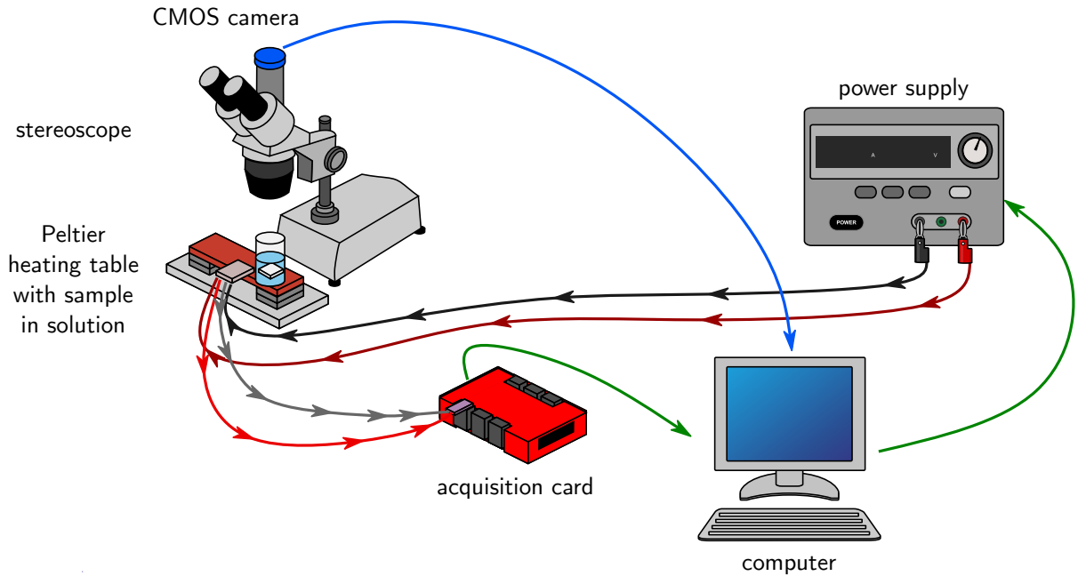
Figure 4.7: Schematics of the experimental setup enabling observation of MgO etching using a stereo microscope and a PID-controlled heater stage. The temperature is controlled with a LabVIEW program by adjusting the current passing through the Peltier cells via feedback mechanism. The temperature near the beaker is measured with a Pt thermistor and retrieved using an acquisition card.
