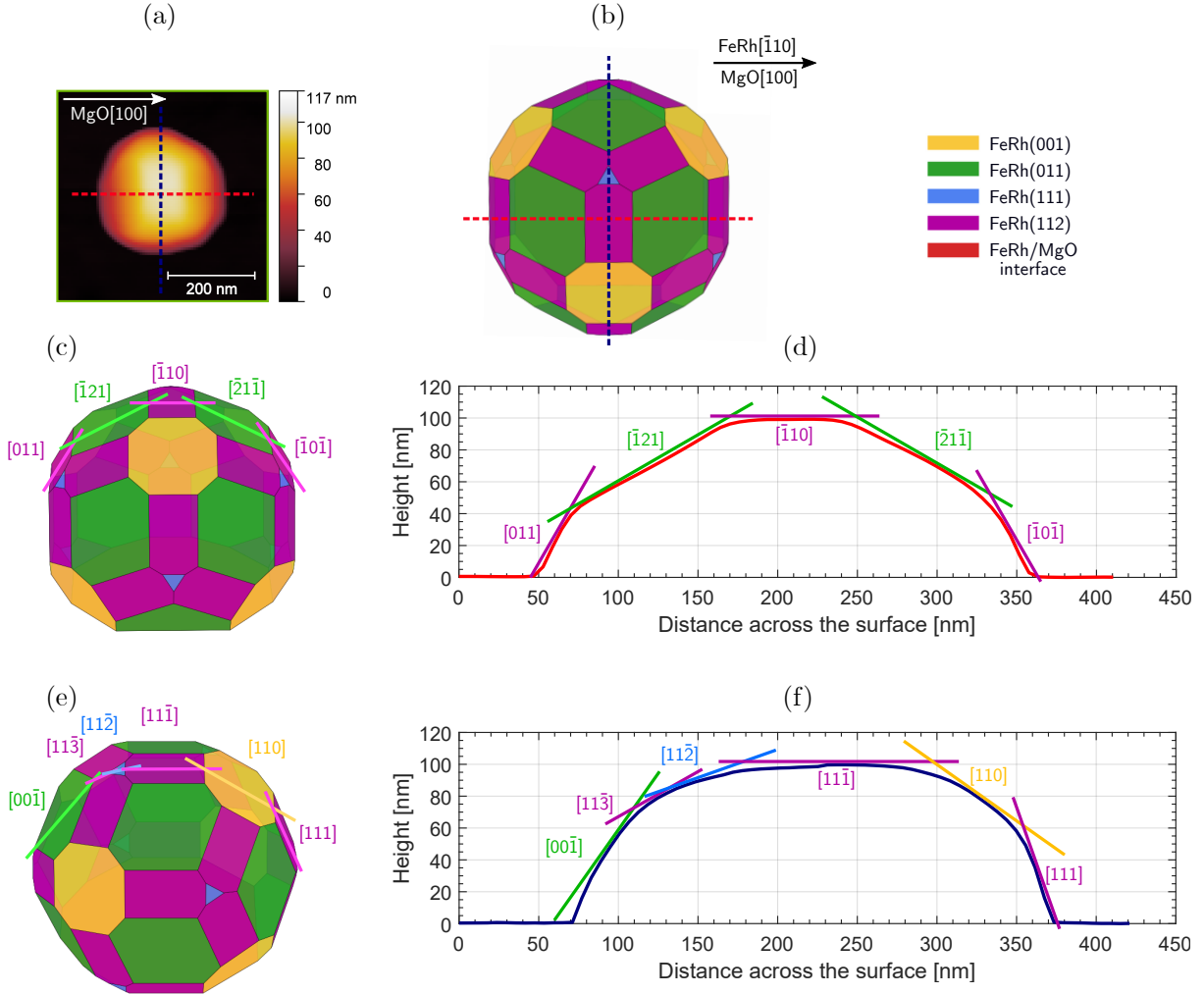
Figure 2.14: Nanoisland shape analysis of FeRh(112) on MgO(011): (a) high-resolution AFM image of a 300-nm-wide island from a region of sample M(011)-16 shown in Figure 2.11a–b. The red and dark blue dashed lines indicate the positions of the line-scans shown in (d) and (f), respectively. (b) Top view of the FeRh(112)/MgO(011) Winterbottom construction, showing a comparable projection of the island shape experimentally observed in (a). The dashed lines indicate the facet paths selected for the analysis. (c) Oblique view of the Winterbottom construction, showing the FeRh lattice directions corresponding to the facet path across the particle as indicated by the red dashed line in (b). (d) The experimental height profile extracted from the linescan along the red dashed line in (a). Superimposed straight lines indicate the facet directions as theoretically extracted from the Winterbottom construction in (b) and (c). (e) Oblique view of the Winterbottom construction, showing the FeRh lattice directions corresponding to the facet path across the particle as indicated by the dark blue dashed line in (b). (f) The experimental height profile extracted from the linescan along the dark blue dashed line in (a). Superimposed straight lines indicate the facet directions as theoretically extracted from the Winterbottom construction in (b) and (e).
