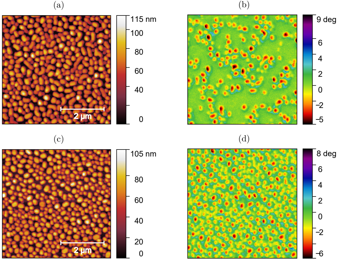
Figure 3.3: AFM (left panel) and MFM (right panel) images for samples grown on \text{Al}_2\text{O}_3(0001) : (a)–(b) sample A(0001)-16; (c)–(d) sample A(0001)-12.
