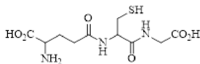
glutathion
