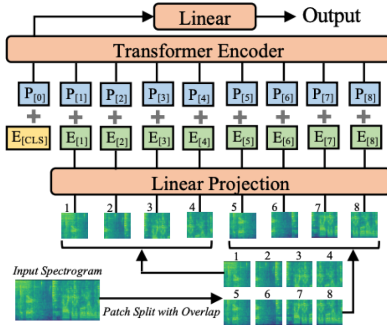
Figure 3.2: Architecture proposed by the authors of AST [13]
