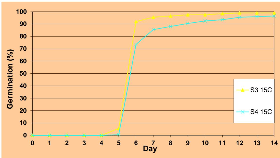
Figure 5: Samples 3 and 4 (all common bean samples). S3 15C = Sample 3 (New Beans – Variety Name Kabulangeti – Less than 6 months old), S4 15C = Sample 4 (Old Beans – Variety Name
