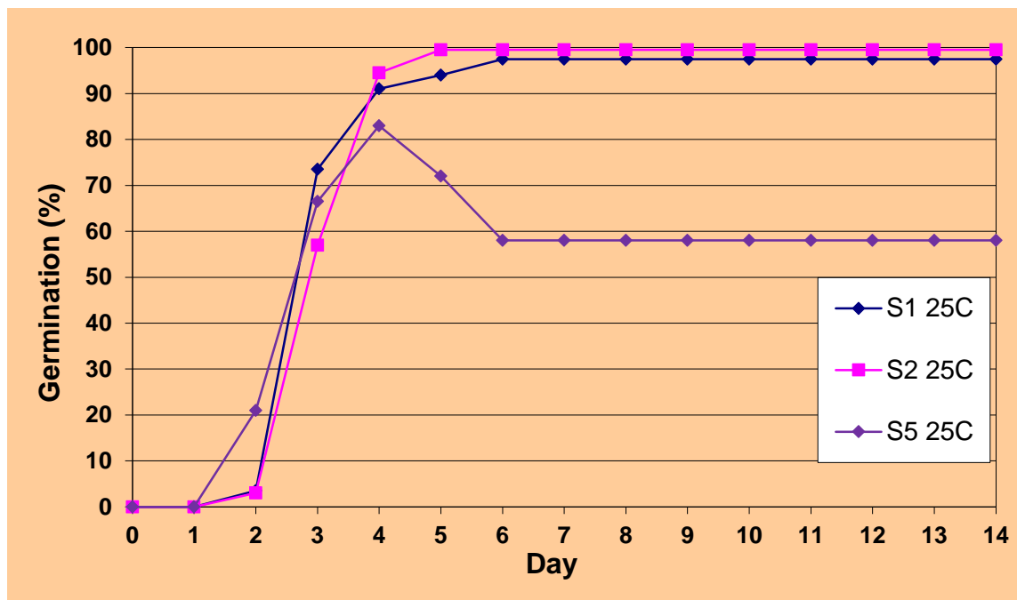
Figure 2: Samples 1, 2 and 5 (all maize samples) at 25 degrees Celsius. S1 25C = Sample 1 (New Maize – Local Maize with Shumba Preservation Dust – Less than 6 months old), S2 25C = Sample 2 (Hybrid Maize – Aminika WH507, Pink in Colour – Treated) and S5 25C = Sample 5 (Old Maize – Local Maize without Preservation Chemicals – 1-year-old). S2, although it was slower in germination for the first 2 days of observation, it was the only seed that eventually achieved 100% germination. It can be seen that S5 records a decrease in germination percentage after the fourth day.
