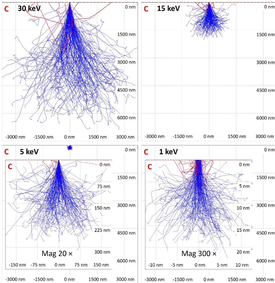
Fig. 2.2: Monte Carlo simulations of electron trajectories in carbon sample with a density of 2.6 \text{ g/cm}^3 for primary electron energies of 30, 15, 5 and 1 keV, respectively. Computed in CASINO 2.4.8.1 [3].
