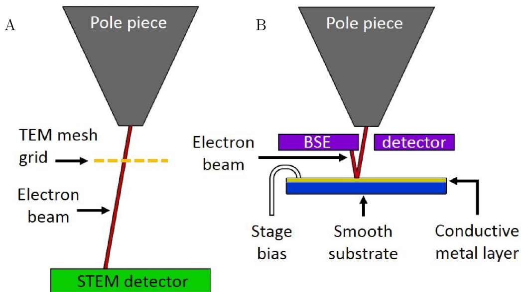
Fig. 10.1: Diagram of energy-dependent calibration of STEM detector (A) and BSE detector (B). Calibration of the BSE detector is performed by primary beam reflection on the biased sample instead of direct imaging used in case of the STEM detector. Taken from [10].
