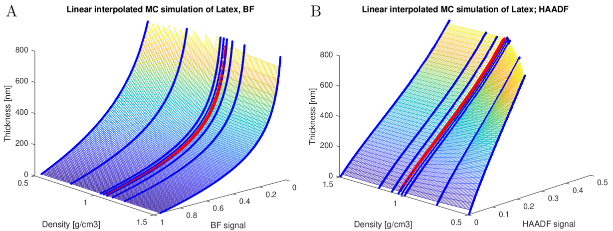
Fig. 4.4: Monte Carlo simulation signal space of latex in BF (A) and HAADF (B). Notice the inverted signal axes. The used density of 1.05 g/cm 3 is highlighted in red. Capturing angles are 0-34 mrad for BF and 167-637 mrad for HAADF.
