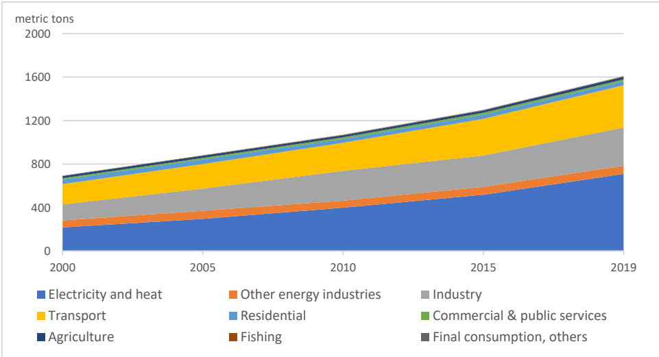
Figure 2 CO2 emissions by sector for ASEAN, 2000-2019 Source: IEA database
