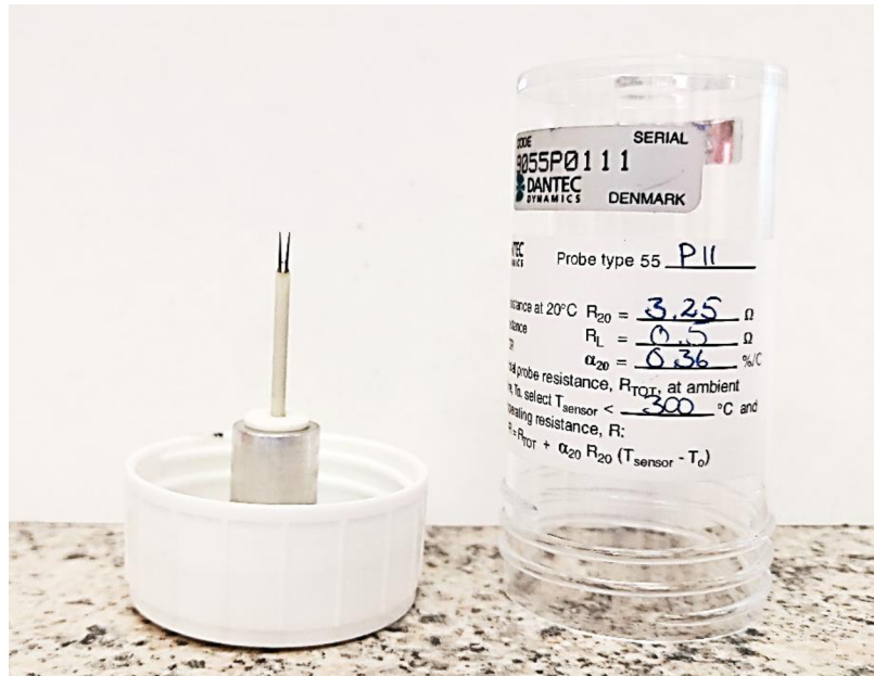
Obr. 3.3 Sonda 55P11
