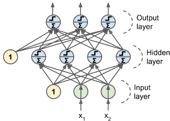
Figure 3.4: Multi-Layer Perceptron [22].
