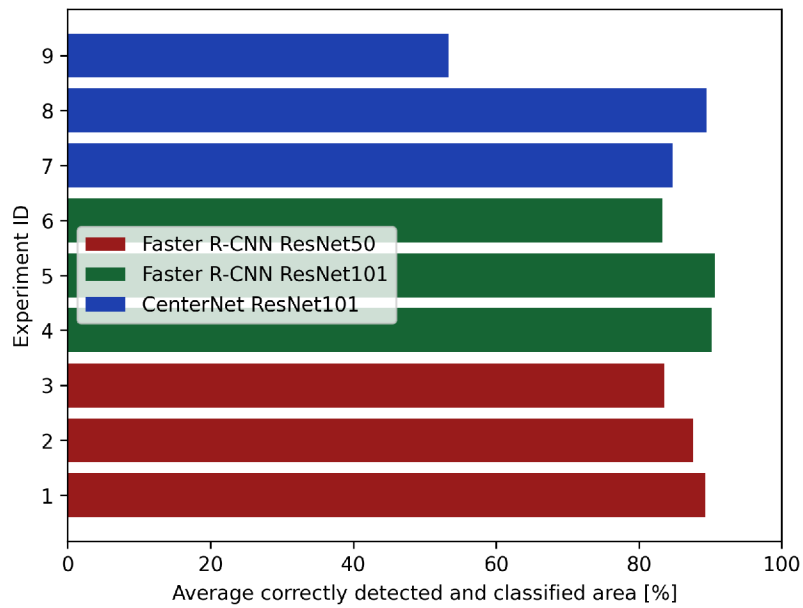
Figure 4.7: Average correctly detected and classified area for each experiment.
