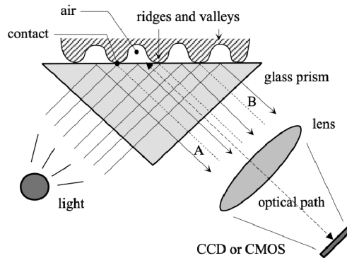
Figure 2.10: Principle of the optical sensor [30].
