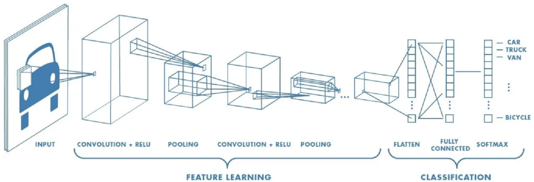
Figure 3.7: A general example of CNN architecture [40].
