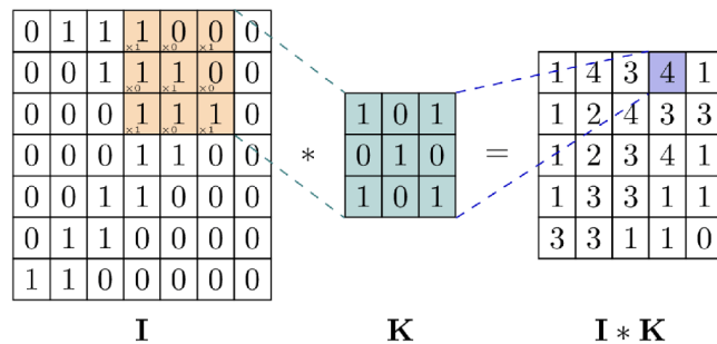
Figure 3.8: Image convolution [37].
