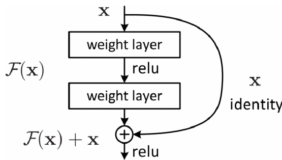
Figure 3.9: Residual block [23].
