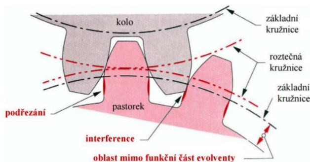
Obr. 24: Interference [8]
