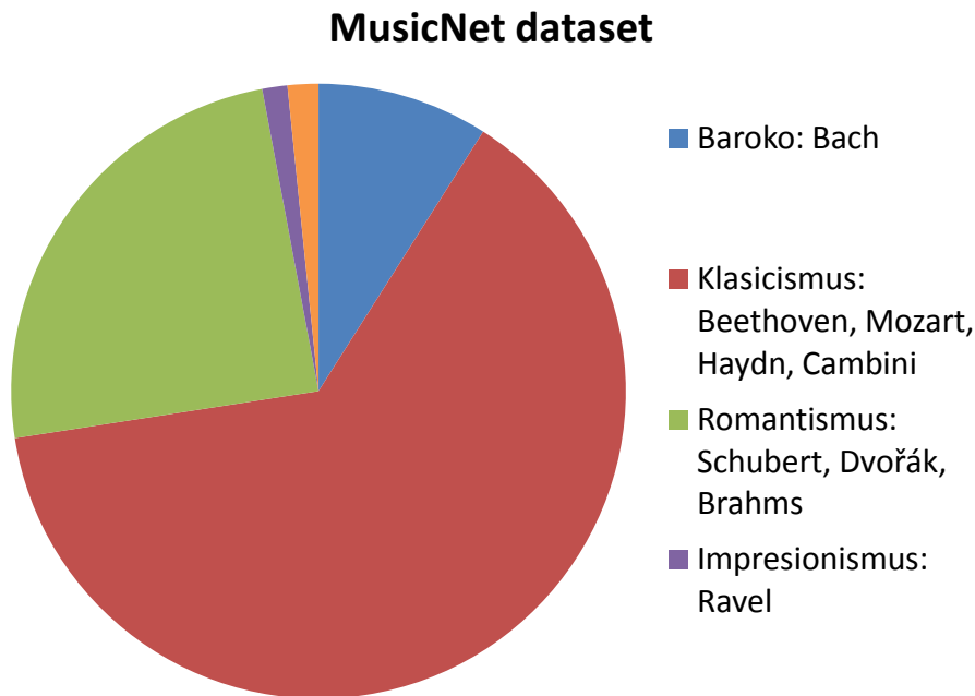
Obr. 2.3: MusicNet dataset
