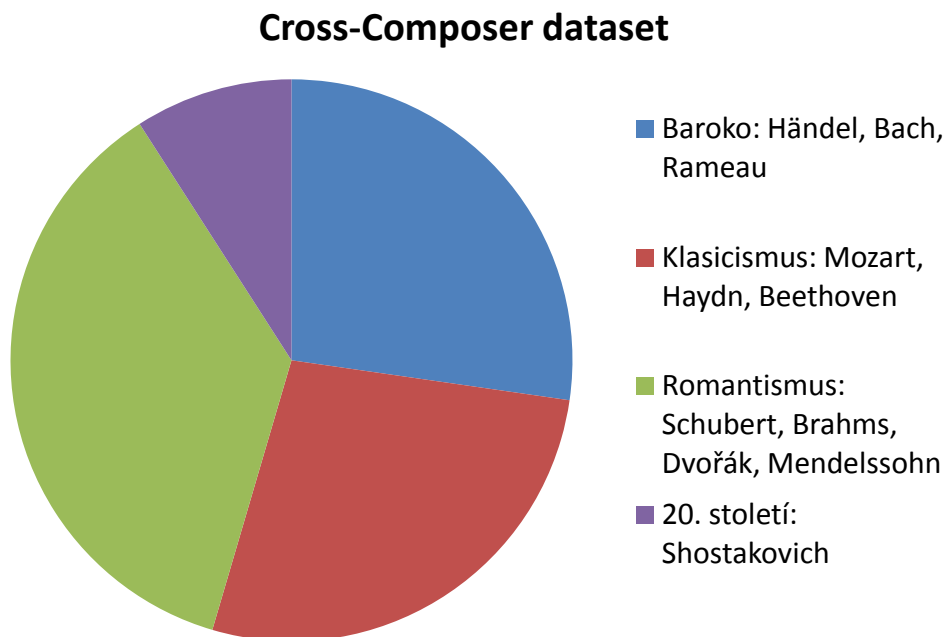
Obr. 2.2: Cross-Composer dataset
