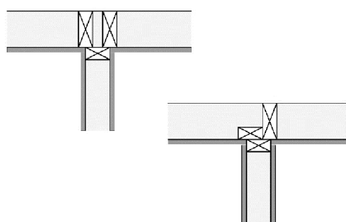
"T" spoj
