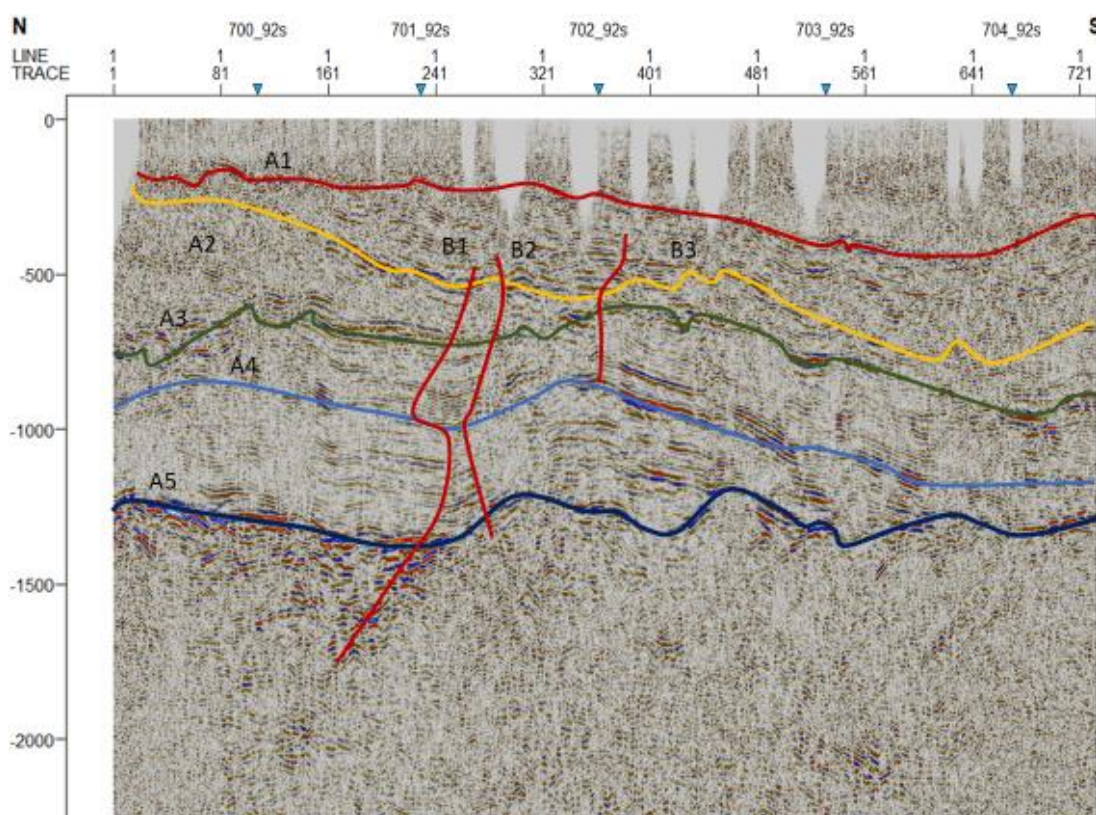
Figure 39 Seismic section 705.
