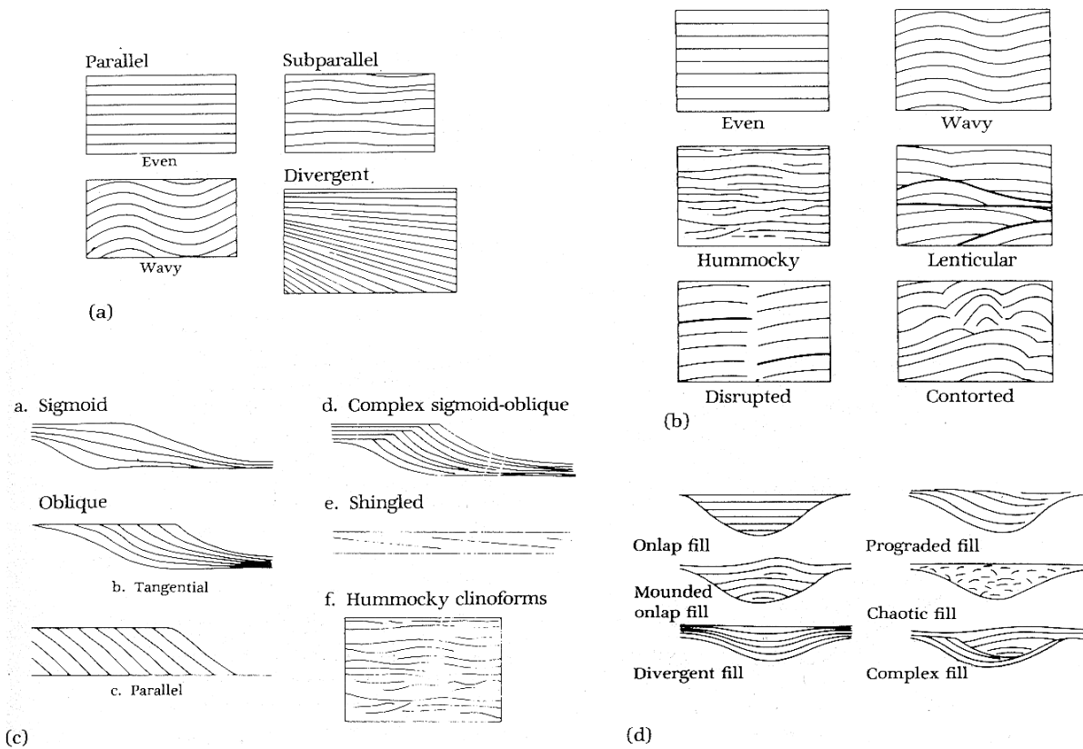
Figure 25 Examples of diagnostic reflection configurations. From Baley, 1991.
