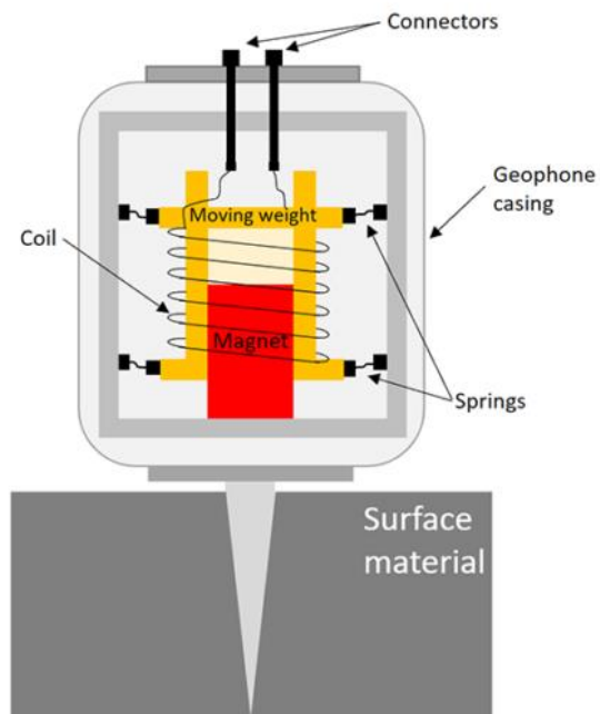
Figure 19 Scheme of geophone (generally 0.707).
