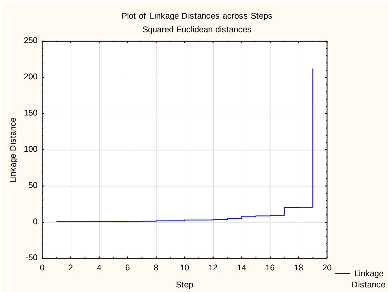
Obr. 7 Plot of Linkage Distances – 2014
