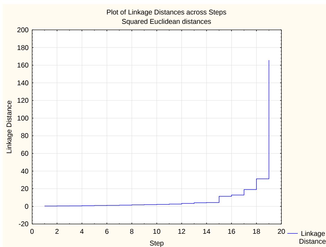
Obr. 5 Plot of Linkage Distances – 2004
