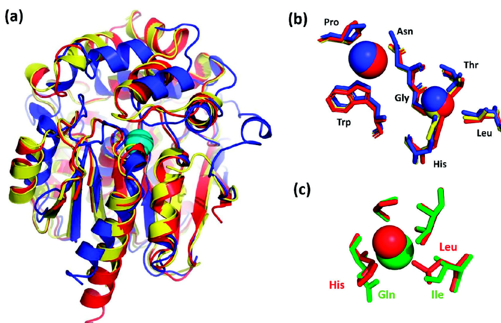
Figure 5. Structural comparison of DbeAΔCl with homologous dehalogenases. (a) DbeAΔCl secondary structure superposition with DhaA and Dh1A. Cα ribbon trace shows elements of the protein secondary structures. The DbeAΔCl is coloured in red; DhaA is coloured in blue; Dh1A is shown in yellow; iodide ion (cyan sphere) is placed in the canonical active site of DbeAΔCl. (b) Superposition of DbeAΔCl, DhaA and Dh1A active sites. Amino acids of DbeAΔCl are shown as red sticks; amino acids of DhaA are shown as blue sticks; amino acids of Dh1A are shown as yellow sticks. The iodide ion and water molecule W11 bound to DbeAΔCl are represented as red spheres; bromide ion and water are shown as blue spheres for the DhaA structure and the single water molecule in the Dh1A is shown as yellow sphere. (c) Superposition of second halide binding site residues of mutant and wild type DbeA. DbeAΔCl amino acids are shown as red sticks; amino acids of DbeAwt are shown as green sticks. Water W71 is shown as red sphere and Cl - ion is shown as green sphere.
