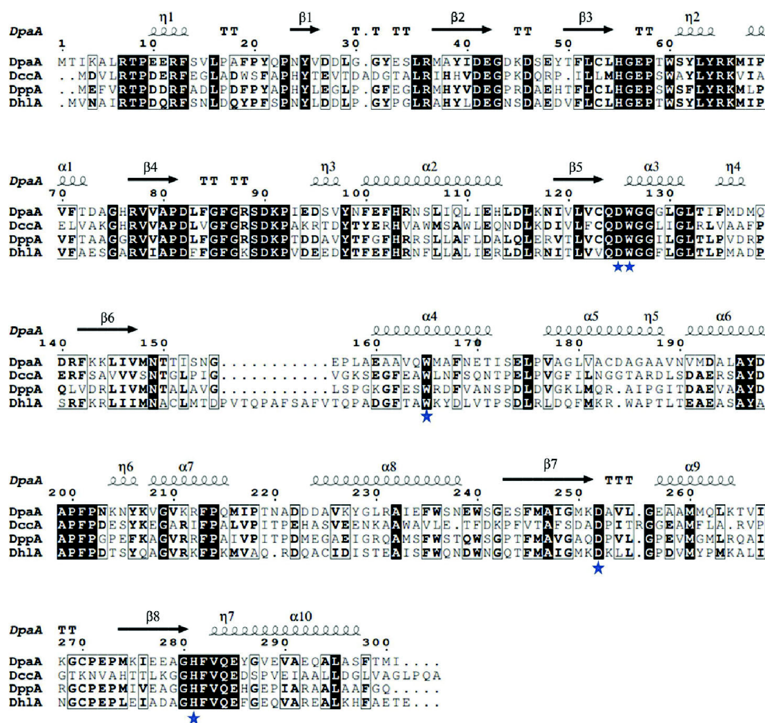
Figure 3 Multiple sequence alignment of the structurally described haloalkane dehalogenases DpaA from Paraglaciecola agarilytica NO2 (PDB entry 7avr), DccA from Caulobacter crescentus (PDB entry 5ers), DppA from Plesiocystis pacifica SIR-I (PDB entry 2xt0) and Dh1A from Xanthobacter autotrophicus GJ10 (PDB entry 2dhc). Catalytic residues are marked by blue stars. Identical residues are presented in white on a black background; similar residues are in bold. Secondary-structure elements of DpaA are shown above the sequences. The alignment was generated with Clustal Omega (Sievers et al. , 2011) and visualized using ESPrpt 3.0 (Robert & Gouet, 2014).
