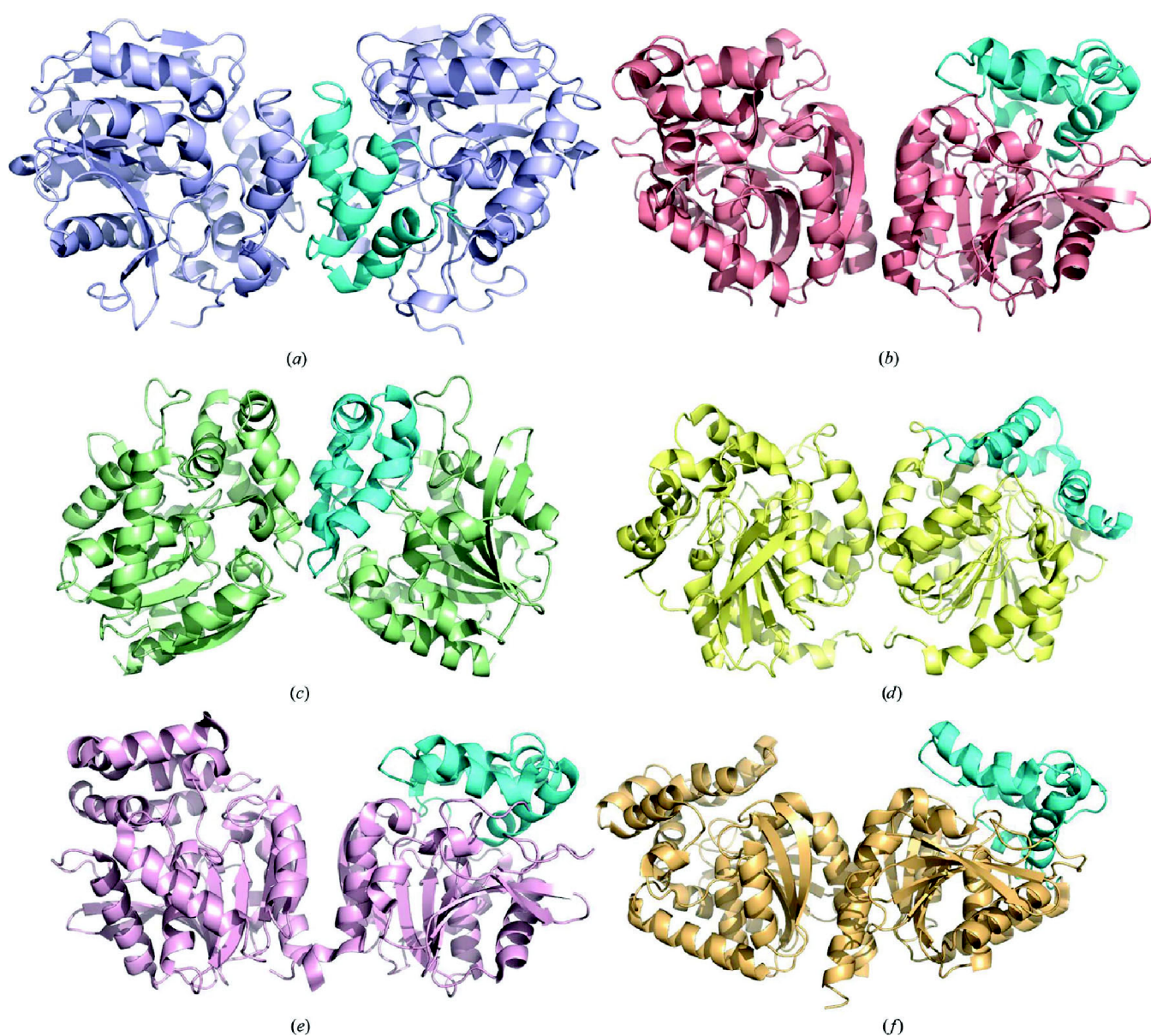
Figure 5 Cartoon models of the overall structures of various haloalkane dehalogenase dimers: (a) DpaA from Paraglaciicola agarilytica NO2 (PDB entry 7avr; this study), (b) DmmA from Moorea producta (PDB entry 3u1t), (c) HanR from Rhodobacteraceae sp. (PDB entry 4brz), (d) DccA from Caulobacter crescentus (PDB entry 5ers), (e) DmxA from Marinobacter sp. (PDB entry 5mxp) and (f) DbeA from Bradyrhizobium elkanii (PDB entry 4k2a). The cap domain is shown in cyan.
