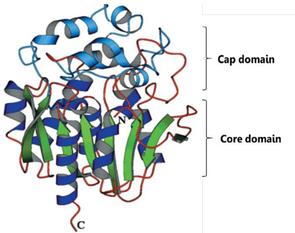
Figure 1. Overview of the tertiary structure of LinB. \alpha -Helices, \beta -sheets and loops forming the core domain are shown in dark blue, green and red, respectively; while the helices and loops from the cap domain are colored in light-blue [11].
