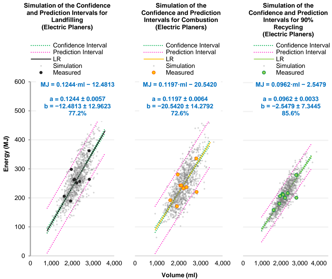
Fig. 6-26 Monte Carlo simulation for Electric Planers (Landfilling, Combustion and Recycling 90%).
