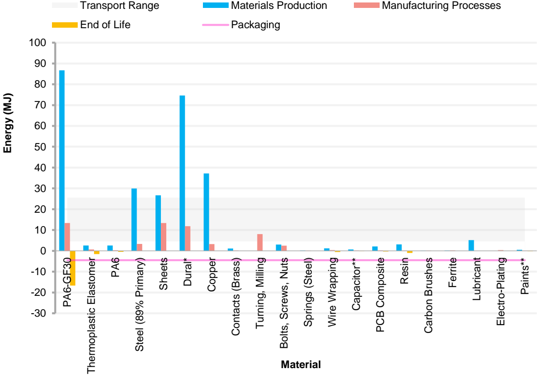
Fig. 6-21 Graph of Reciprocating Saw (Combustion) – Example of LCA profile (RS1).
