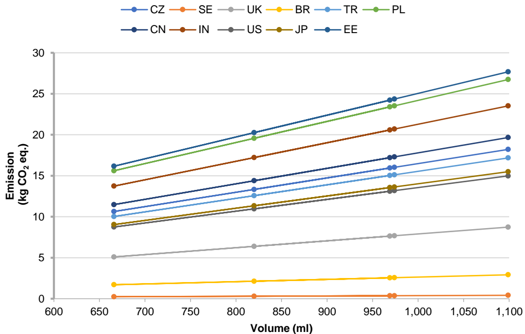
Fig. 6-37 Graph of designed angle grinders with dependency volume and emissions kg CO 2 eq. per selected countries.
