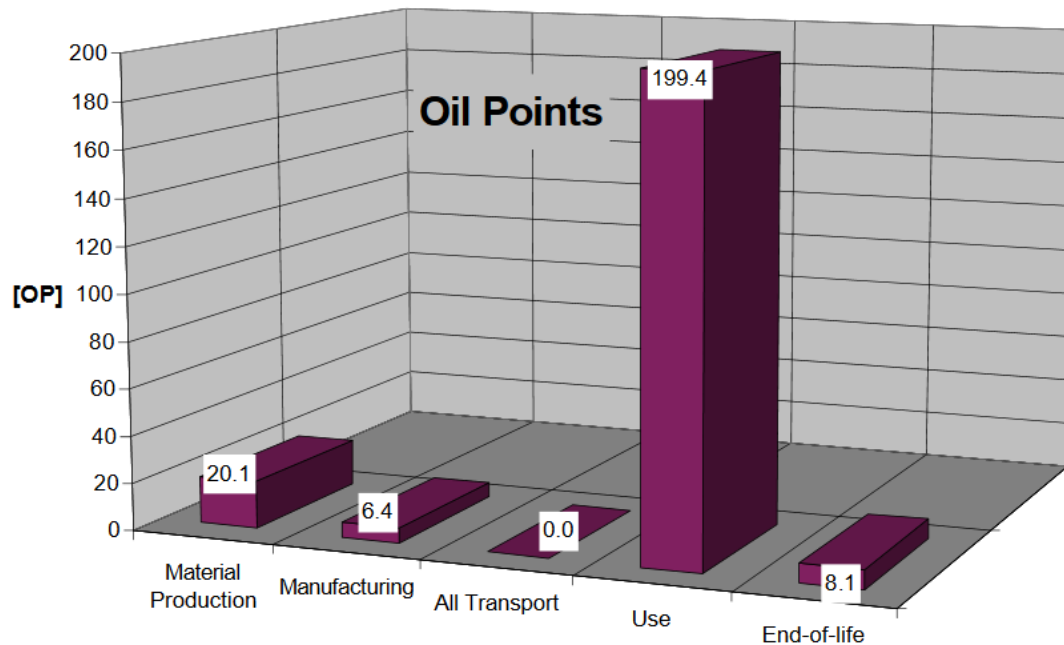
Fig. 2-13 Life cycle according to OP for an electric vacuum cleaner [12].
