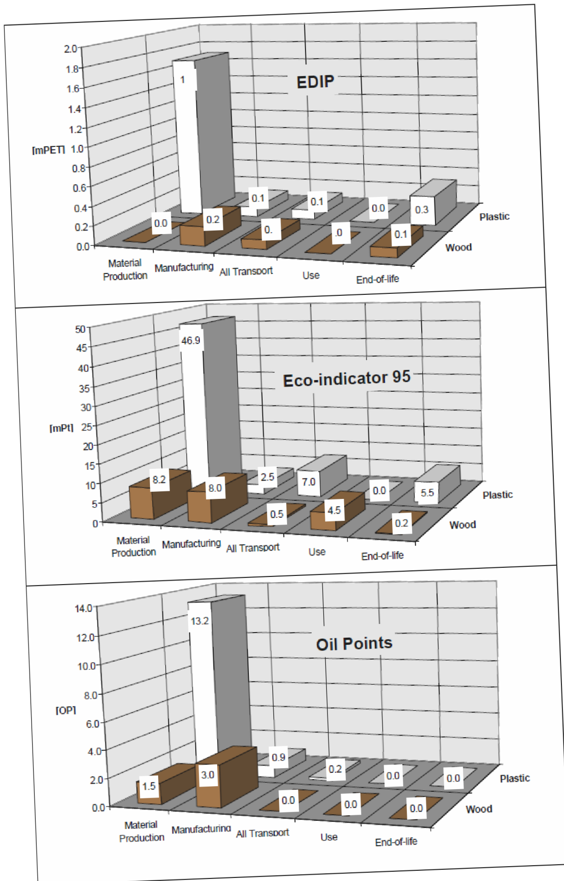
Fig. 2-21 Graphical comparison of different methods for the production of a plastic window [5].
