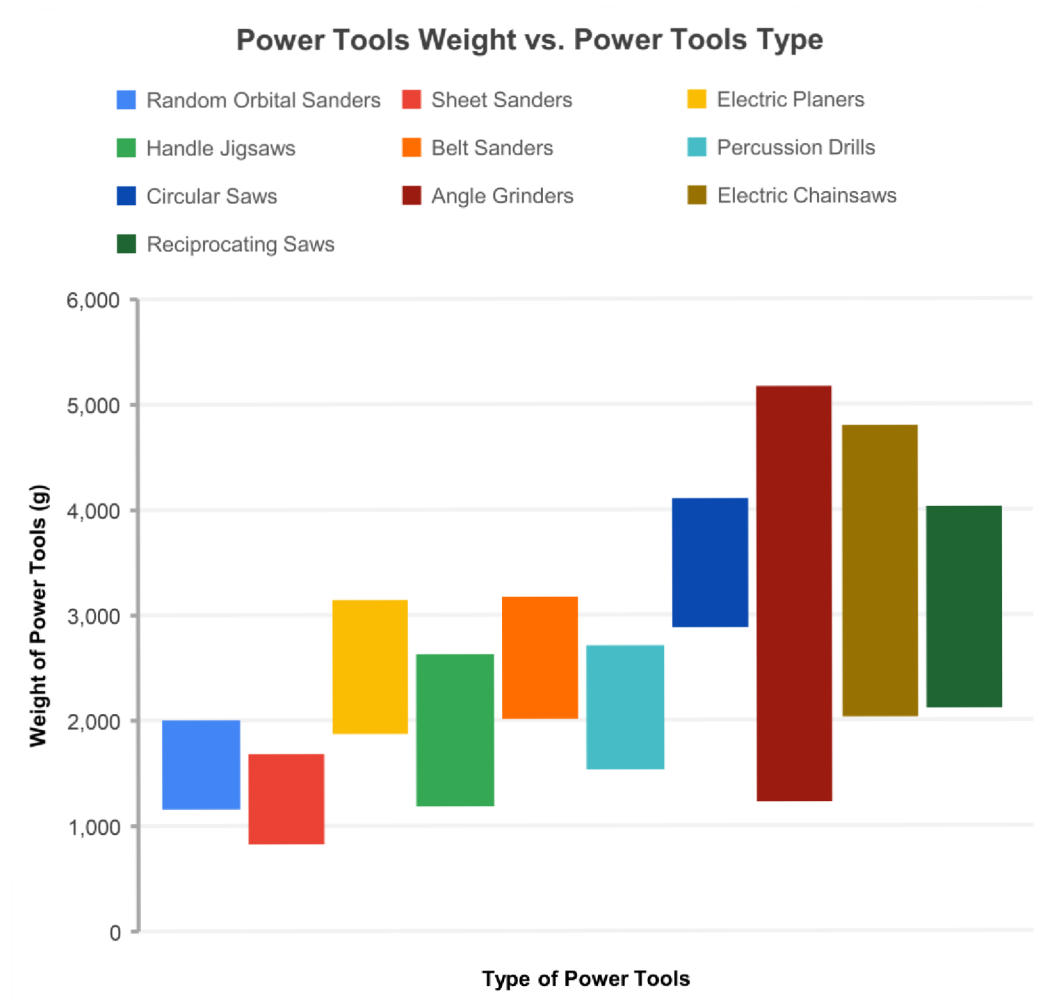
Fig. 6-7 Graph of weight versus power tools type.
