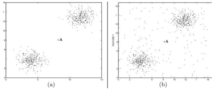
Figure 3: Point A is undoubtedly an outlier in the first graph, but in the second, it is highly subjective to tell[8]
