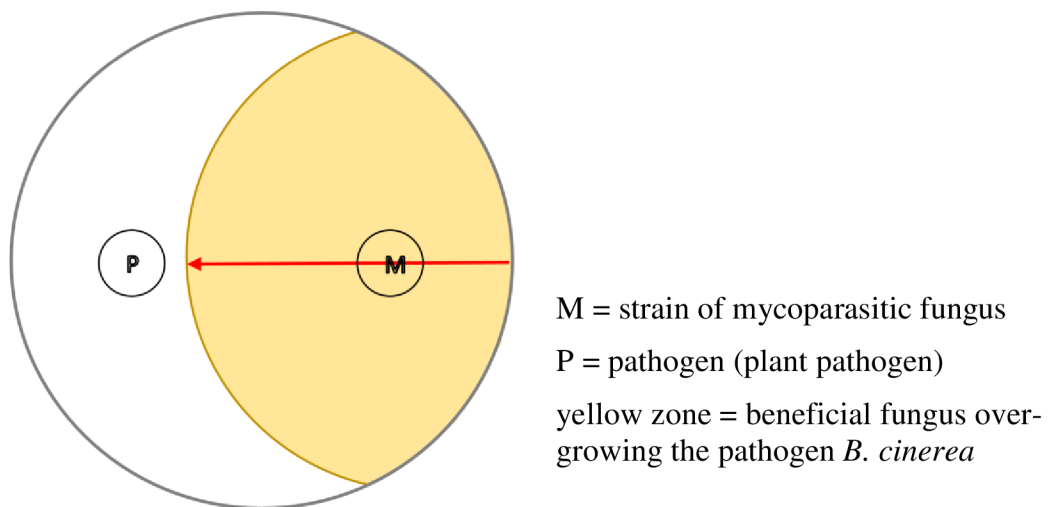
Figure 2. Measurement of mycoparasitic zone between beneficial fungi and B. cinerea
