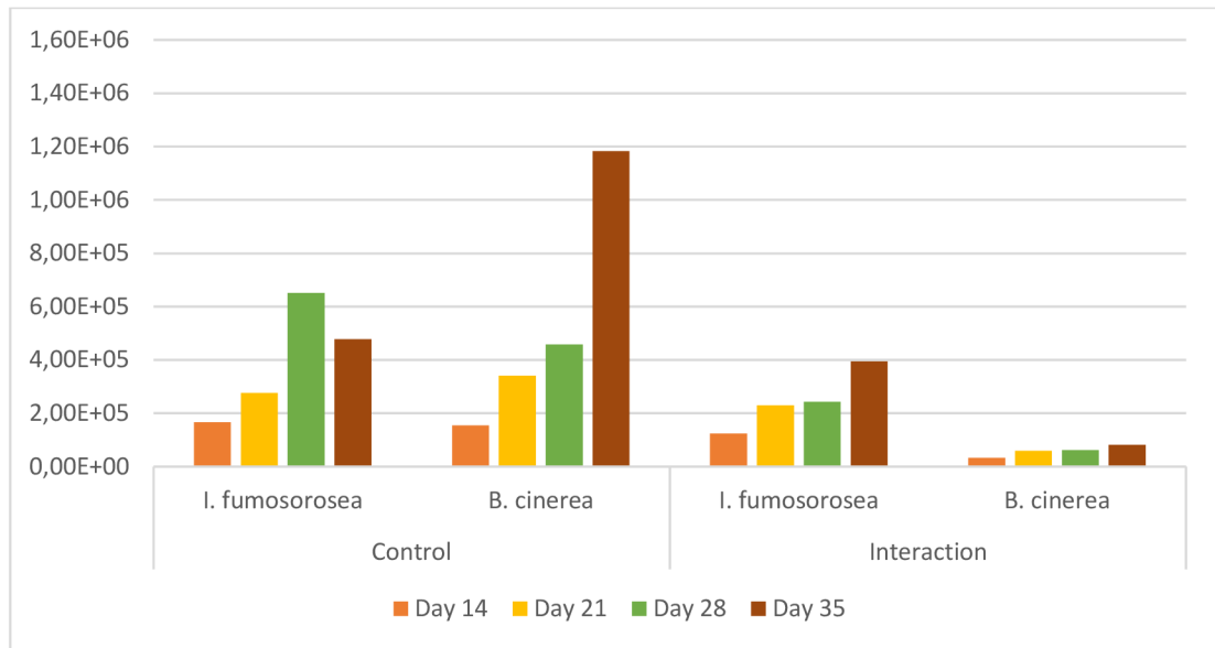
Figure 11: Evaluation of spore production in the interaction between entomopathogenic fungus Isaria fumosorosea and plant pathogen Botrytis cinerea in comparison with control variants
