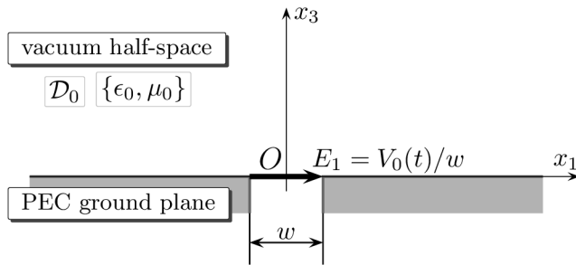
Figure 6.1: Configuration with indication of the aperture feeding.
