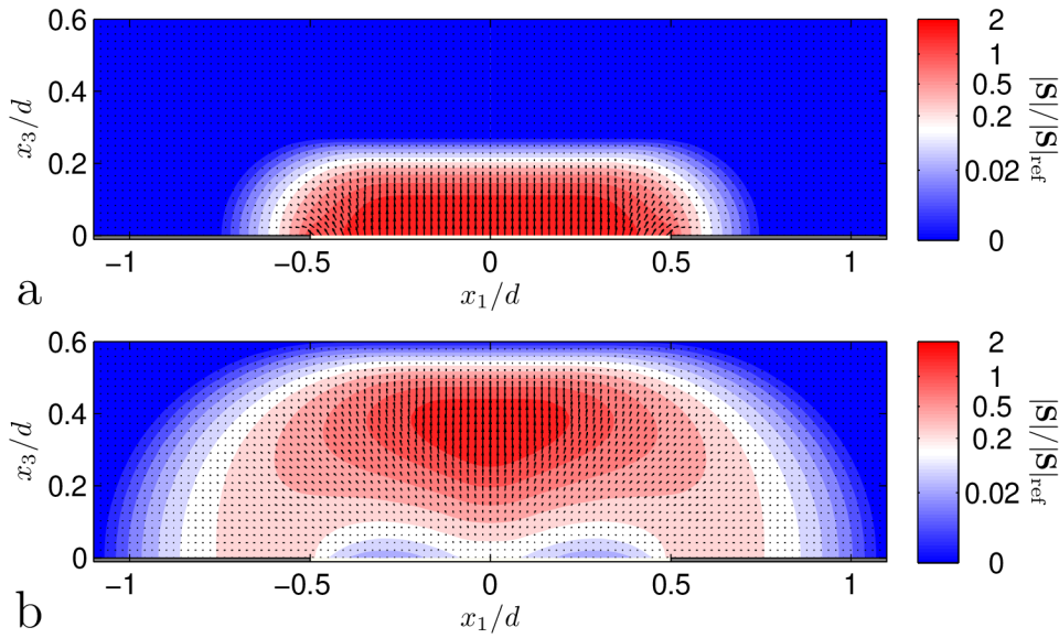
Figure 8.11: Normalized Poynting vector of the EM field at (a) c_0t/d = 0.55 ; (b) c_0t/d = 1.21 . Slab thickness versus slot width is d/w = 1 and electromagnetic parameters of the dielectric slab are \{\epsilon_1, \mu_1\} = \{4\epsilon_0, \mu_0\} . Parameters of the excitation pulse are c_0t_w/d = 0.9236 , \nu = 2 .
