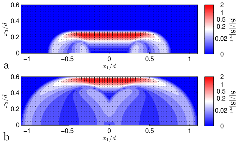
Figure 8.12: Normalized Poynting vector of the EM field at (a) c_0t/d = 0.55 ; (b) c_0t/d = 1.21 . Slab thickness versus slot width is d/w = 1 and electromagnetic parameters of the dielectric slab are \{\epsilon_1, \mu_1\} = \{4\epsilon_0, \mu_0\} . Parameters of the excitation pulse are c_0t_w/d = 0.1847 , \nu = 2 .
