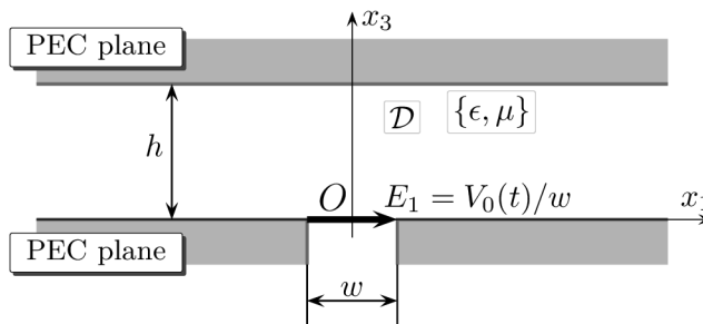
Figure 7.1: Configuration with indication of the aperture feeding.
