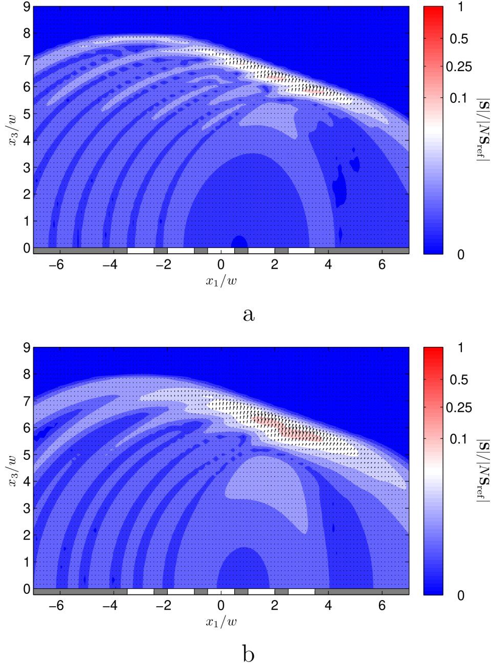
Figure 6.9: Normalized Poynting vectors of EM fields at c_0 t/w = 8 for an array of N = 5 equally spaced slots of width w and spacing (a_{n+1} - b_n)/w = 0.5 , excited with c_0(T_{n+1} - T_n)/w = 0.5 time delays for n = \{1, \dots, 4\} and with two sets of excitation pulses with different spatial supports. (a) c_0 t_w = 0.5542w ; (b) c_0 t_w = 1.1084w .
