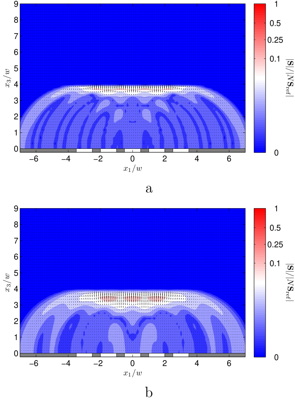
Figure 6.4: Normalized Poynting vectors of EM fields at c_0 t / w = 4 for an array of N = 5 equally spaced slots of width w and spacing (a_{n+1} - b_n) / w = 0.5 for n = \{1, \dots, 4\} , excited with zero time delays and with two sets of excitation pulses with different spatial supports. (a) c_0 t_w = 0.5542w ; (b) c_0 t_w = 1.1084w .
