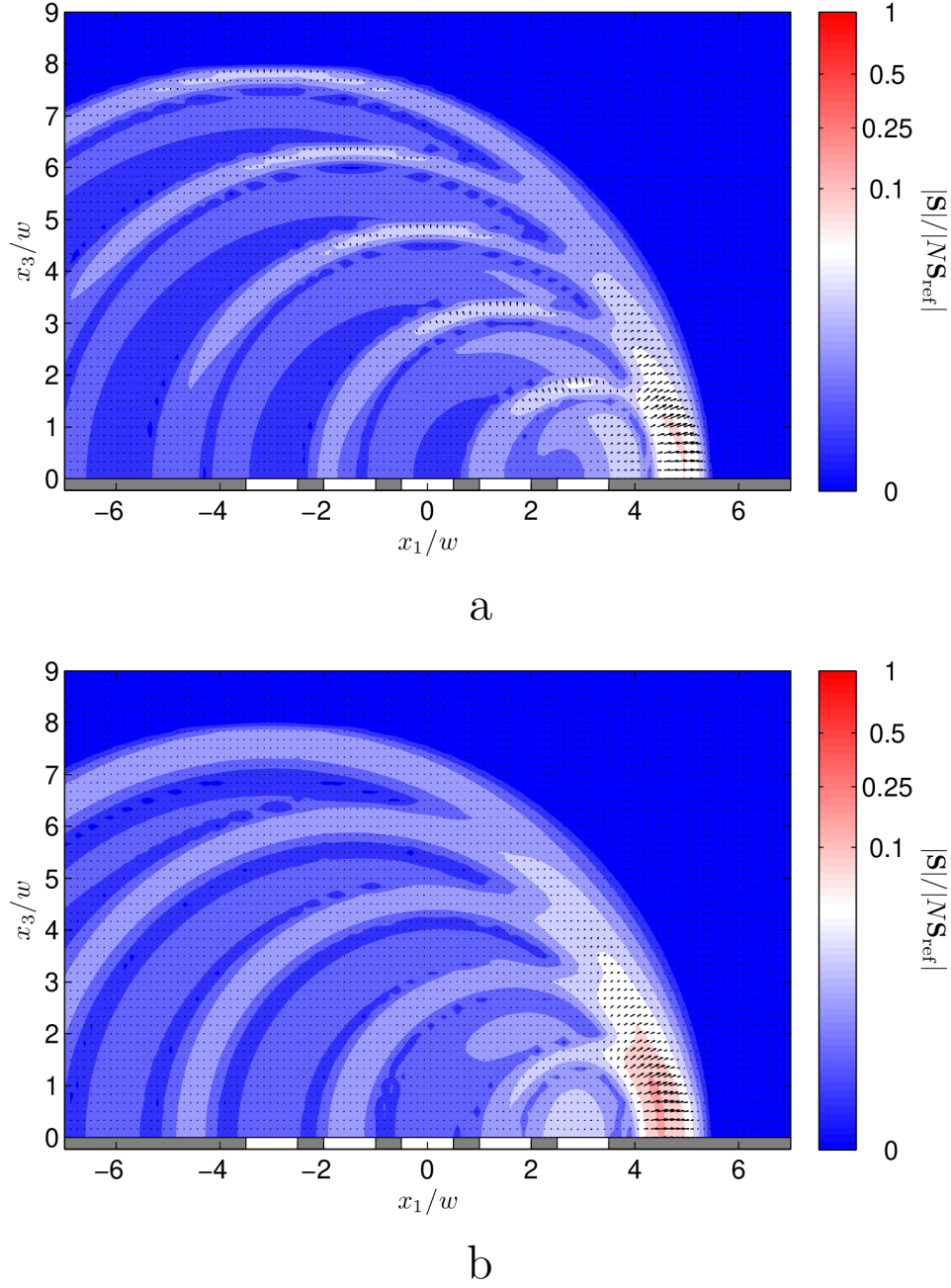
Figure 6.11: Normalized Poynting vectors of EM fields at c_0 t/w = 8 for an array of N = 5 equally spaced slots of width w and spacing (a_{n+1} - b_n)/w = 0.5 , excited with c_0(T_{n+1} - T_n)/w = 1.5 time delays for n = \{1, \dots, 4\} and with two sets of excitation pulses with different spatial supports. (a) c_0 t_w = 0.5542w ; (b) c_0 t_w = 1.1084w .
