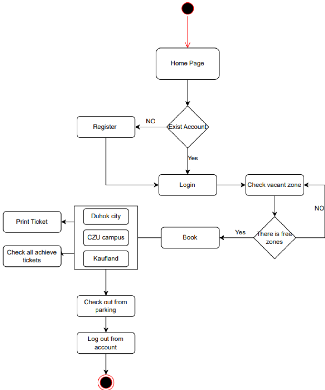
Figure 14: Activity diagram of System operation
