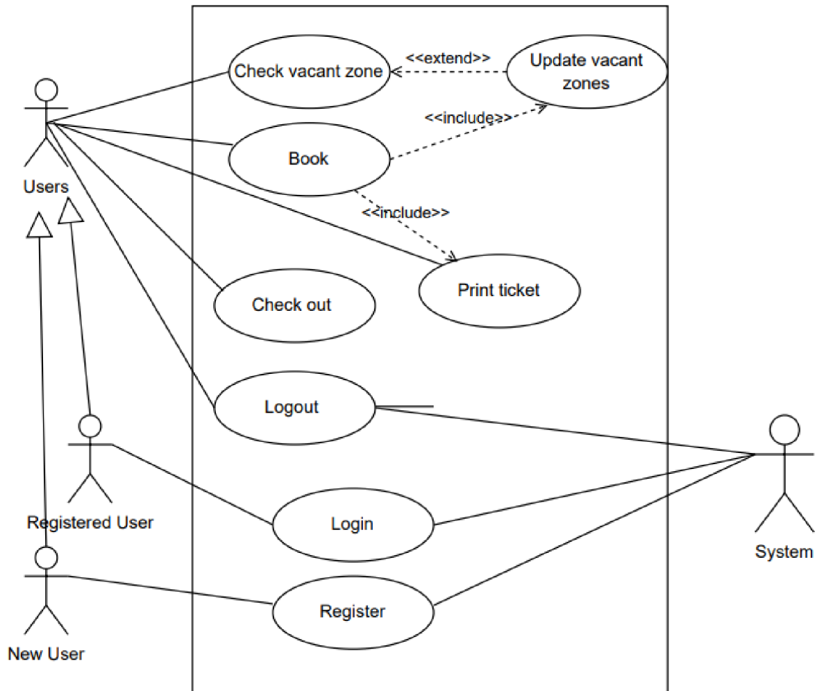
Figure 12: System Use case
