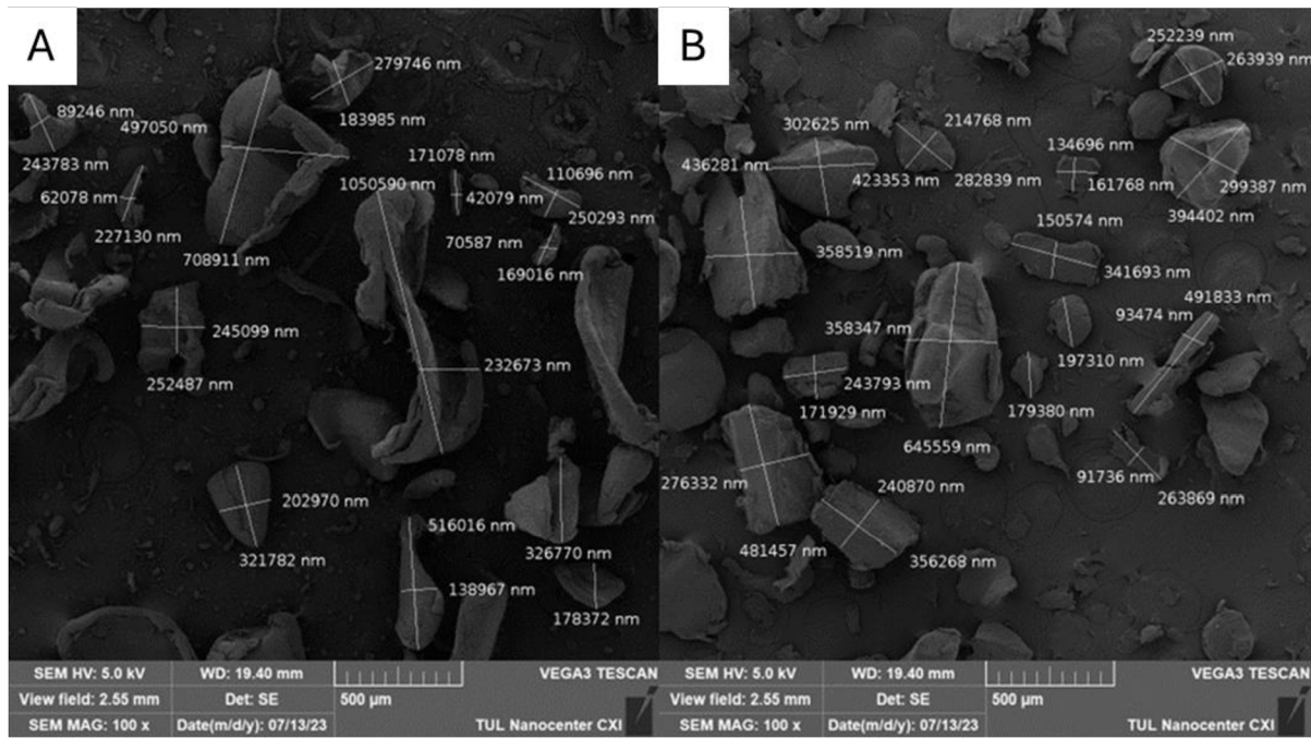
Figure 4.9: SEM and measurement from ImageJ, (A) PET, (B) HDPE.
