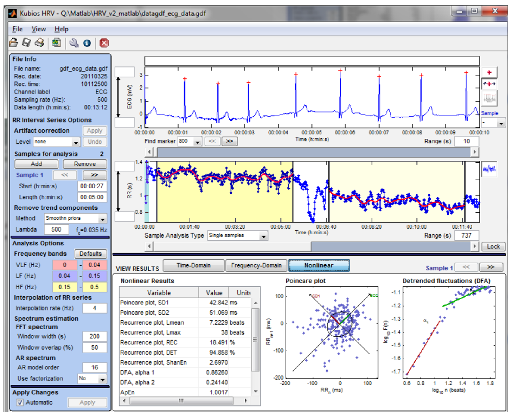
Obr. 2.11: Program KubiosHRV
