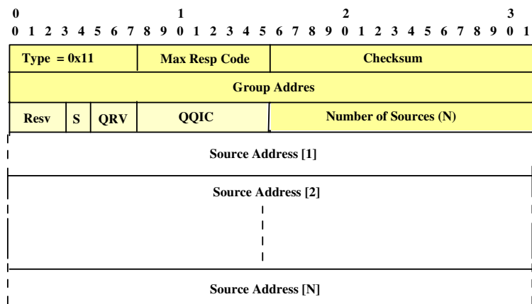
Obr. 8: Zpráva Membership Query [12]
