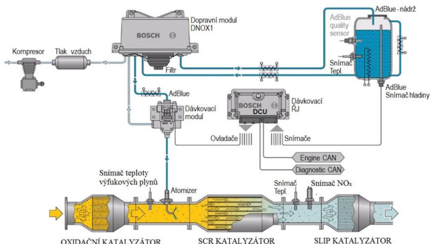
Obr. 11 Bosch denoxtronic [25]
