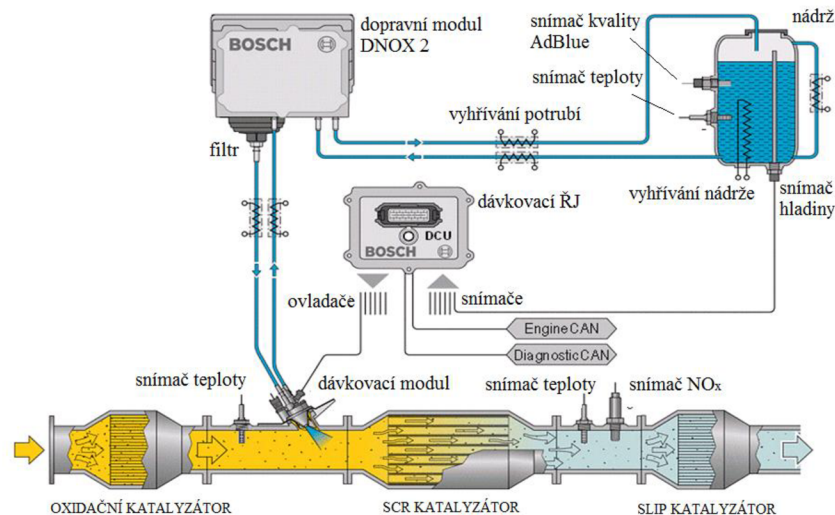
Obr. 14 Bosch denoxtronic 2.1 [25]
