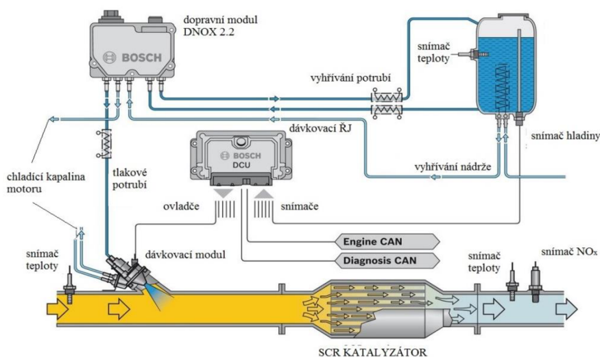
Obr. 17 Bosch denoxtronic 2.2 [27]
